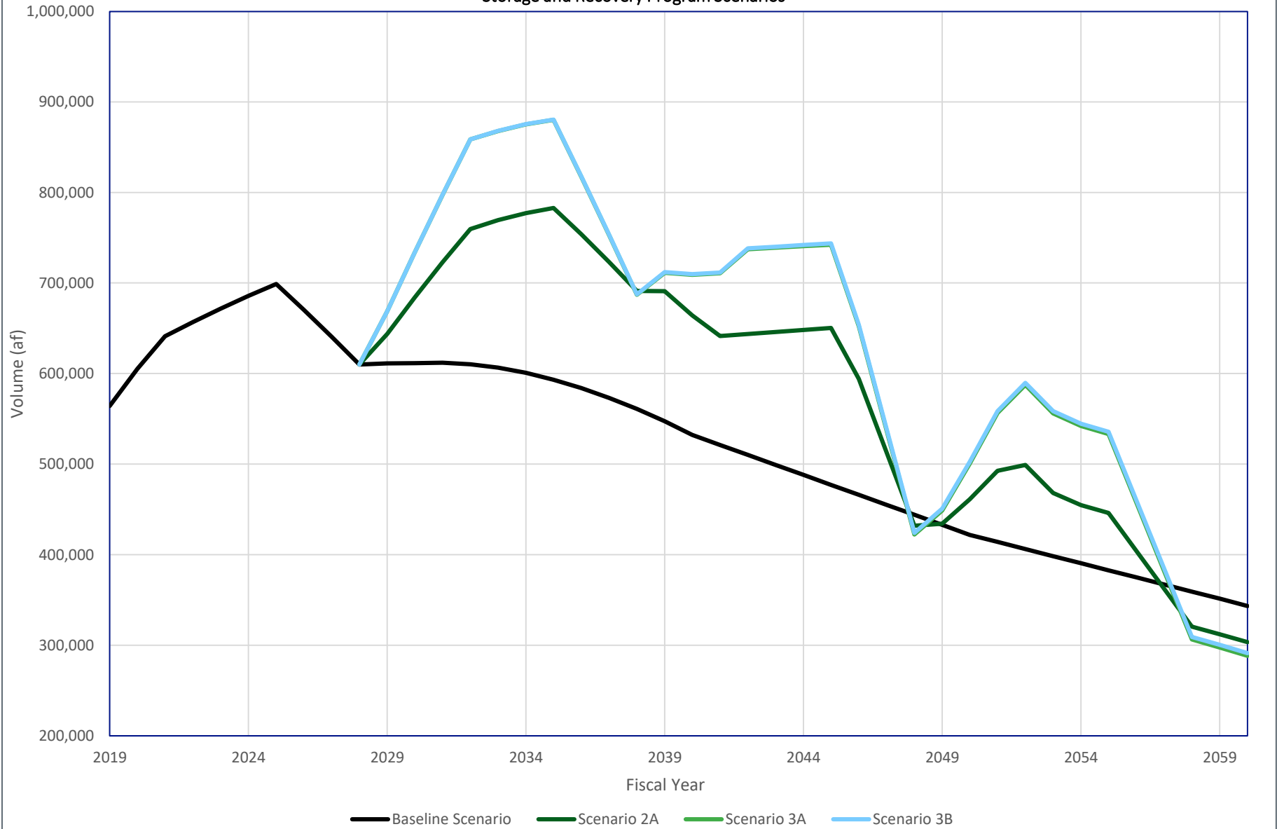
Figure 3-2. Simulated End-of-Year Volume in Managed Storage for the Baseline Scenario and Storage and Recovery Program Scenarios
