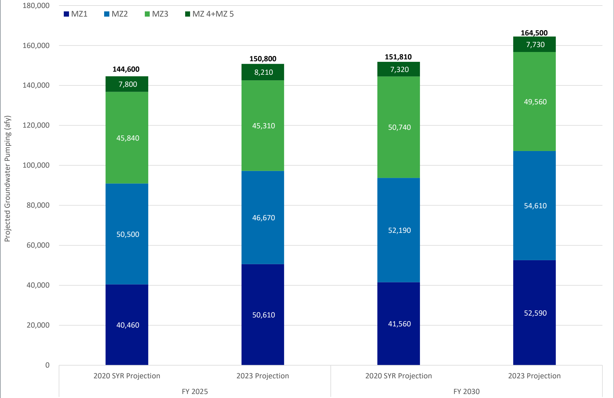
Figure 2-5. Comparison of 2020 SYR Projection versus 2022 Projection for Groundwater Pumping by Management Zone, FY 2025-2030
