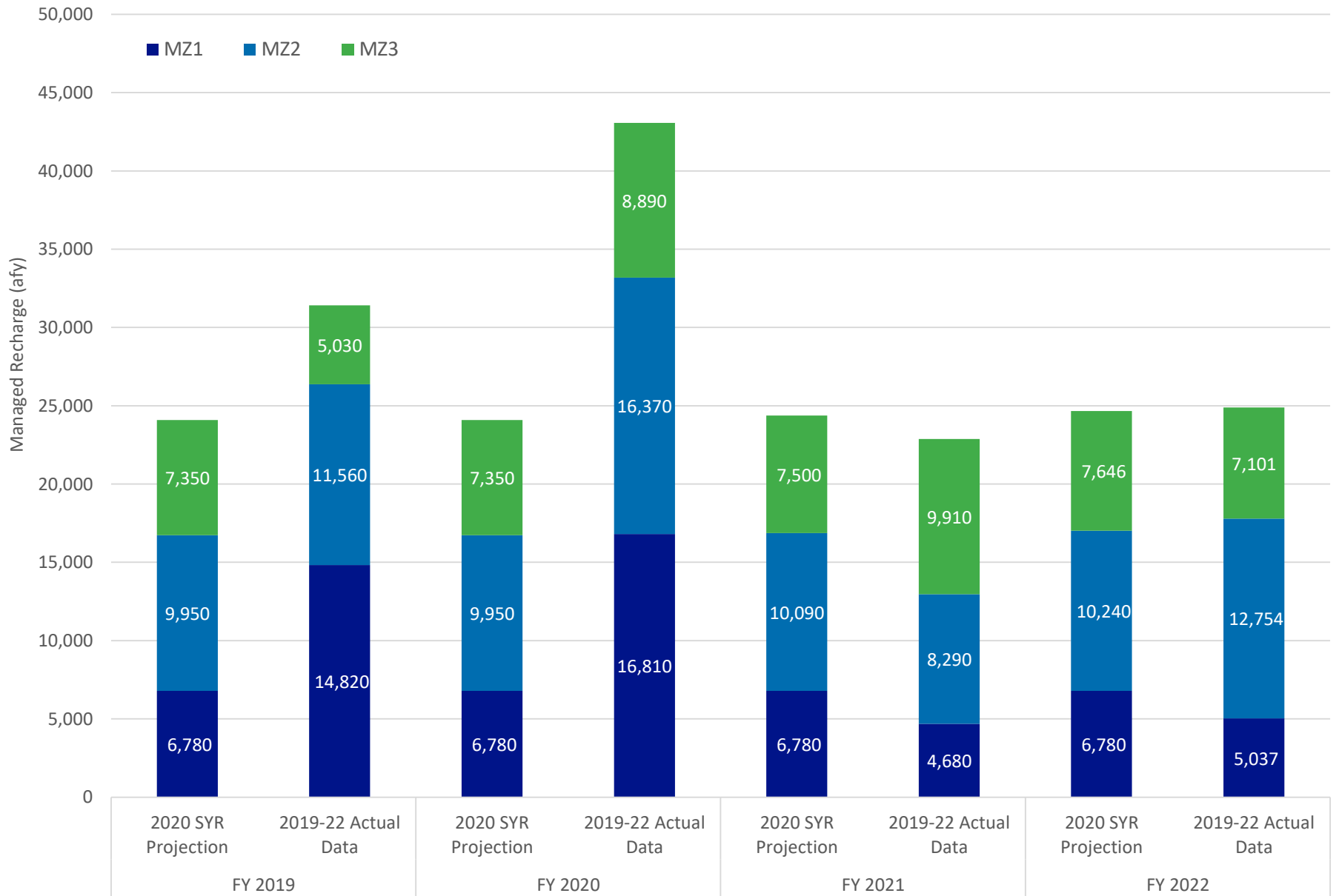
Figure 4-3. Comparison of 2019-22 Actual Data versus 2020 SYR Projection for Managed Recharge by Management Zone, FY 2019-2022
