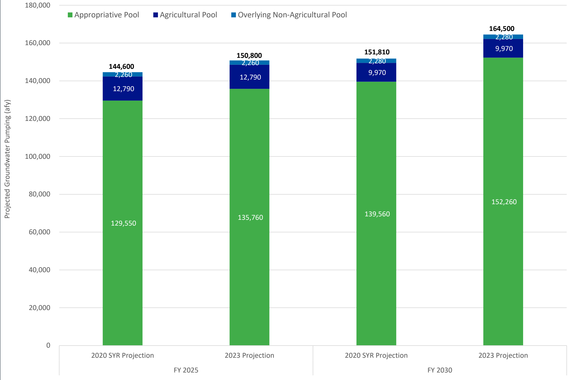
Figure 2-4. Comparison of 2020 SYR Projection versus 2023 Projection for Groundwater Pumping by Pool, FY 2025-2030
