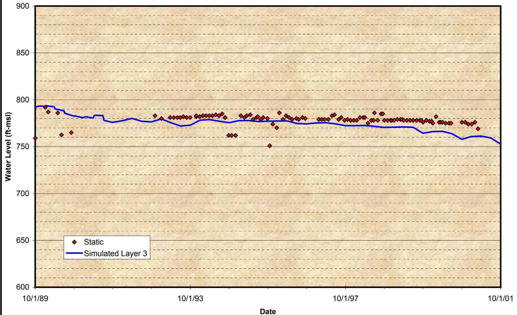
Figure A-4 Comparison of Groundwater Model Projected Time Histories at Wells for the Calibration Period Fontana Water Company – No. F31A
