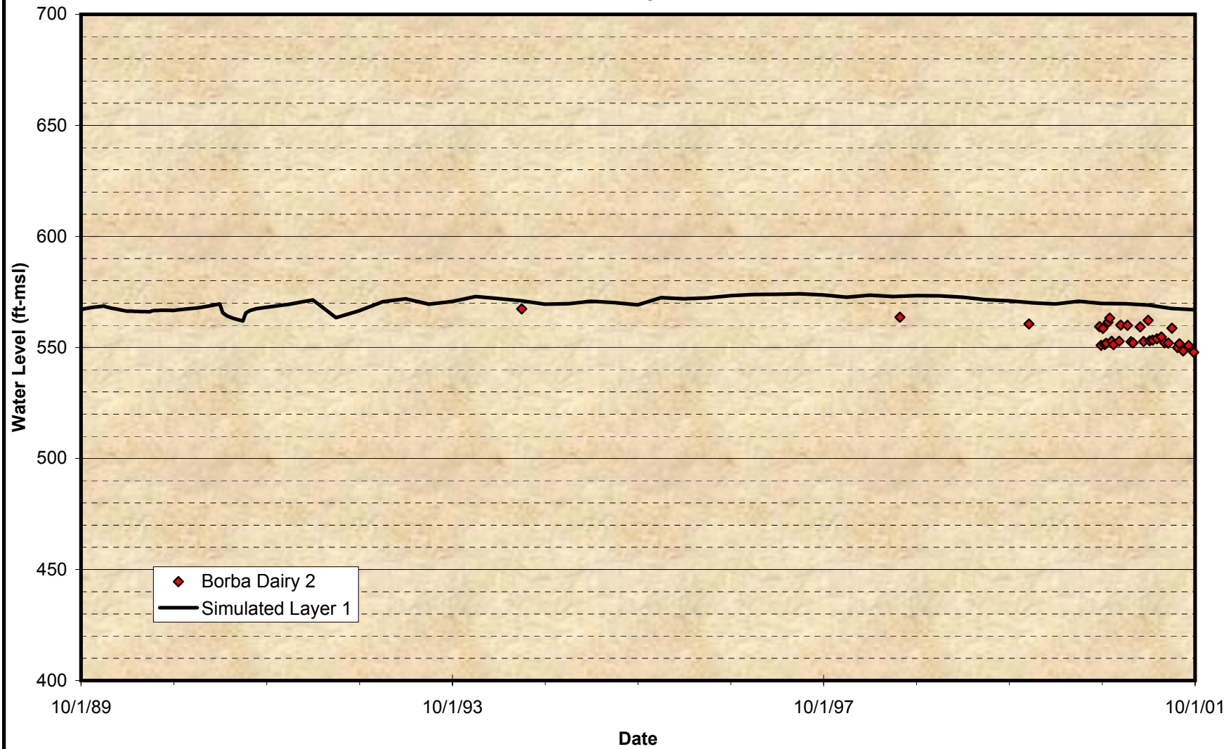
Figure A-35 Comparison of Groundwater Model Projected Time Histories at Wells for the Calibration Period Borba Dairy – No. 2
