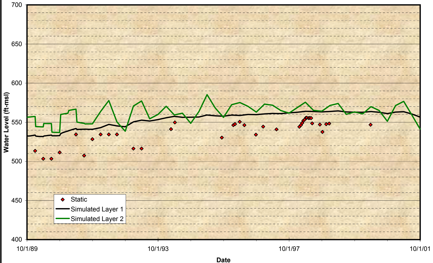
Figure A-24 Comparison of Groundwater Model Projected Time Histories at Wells for the Calibration Period CIM – No. 9
