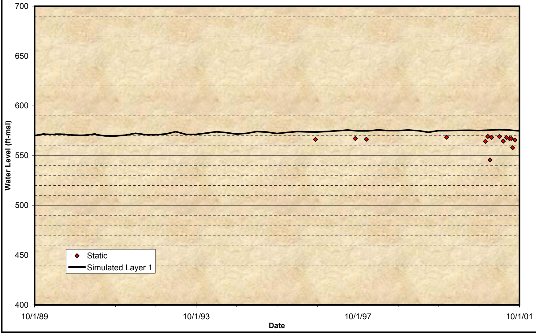
Figure A-33 Comparison of Groundwater Model Projected Time Histories at Wells for the Calibration Period Excelsior
