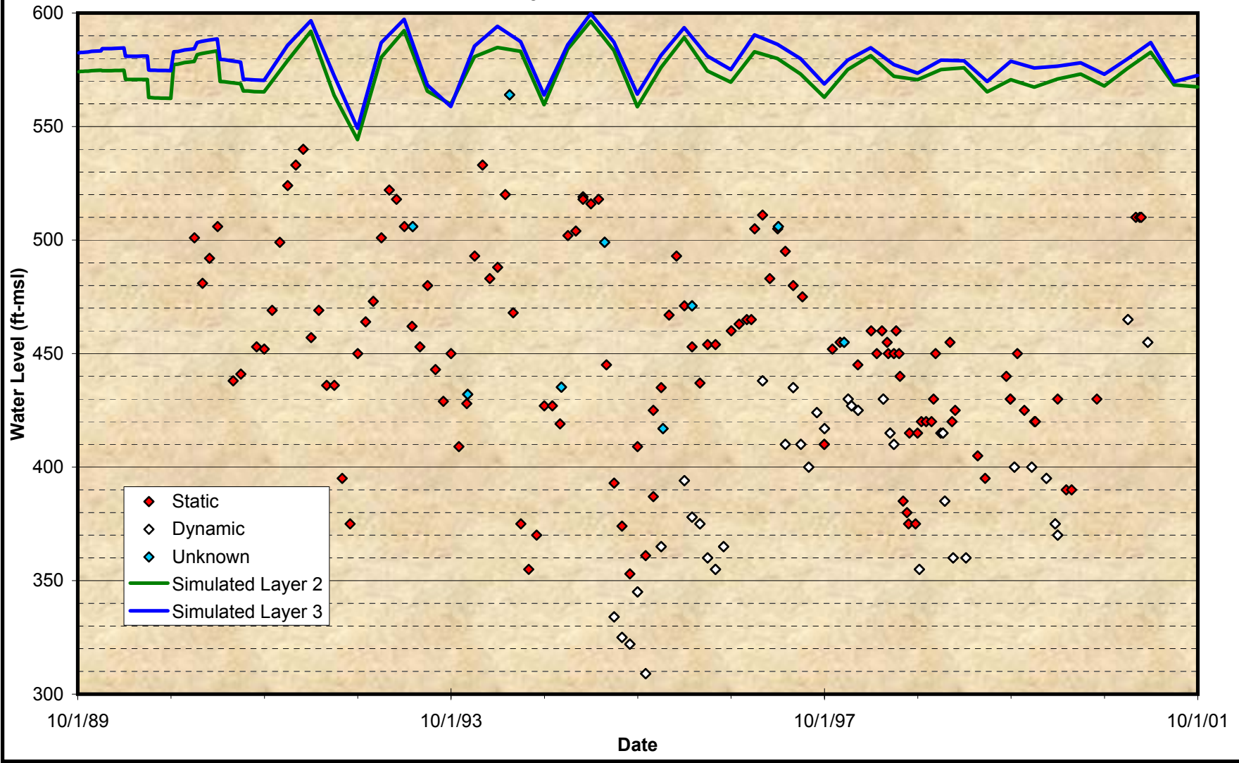
Figure A-26 Comparison of Groundwater Model Projected Time Histories at Wells for the Calibration Period City of Chino Hills – No. 17
