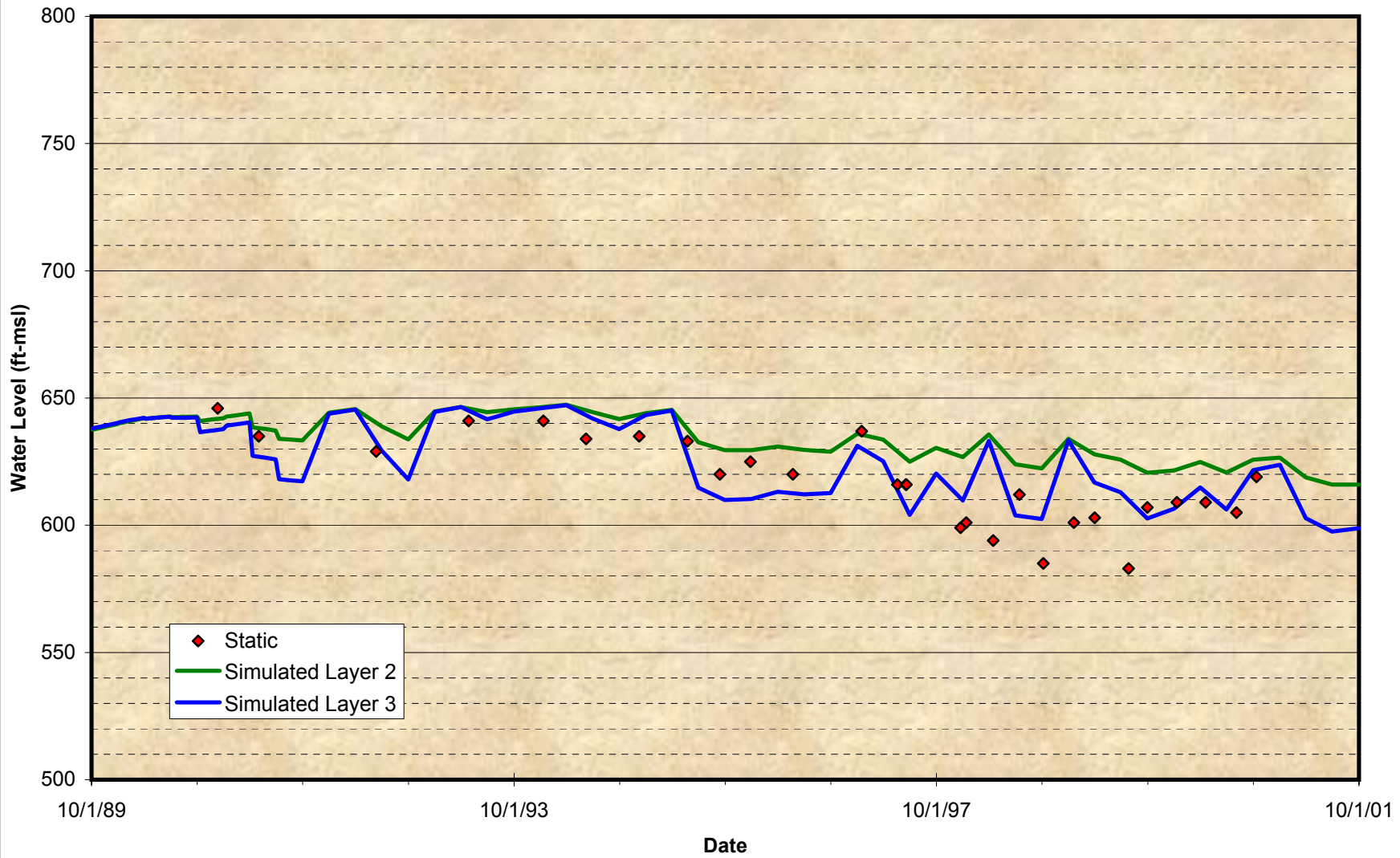
Figure A-11 Comparison of Groundwater Model Projected Time Histories at Wells for the Calibration Period City of Ontario – No. 36
