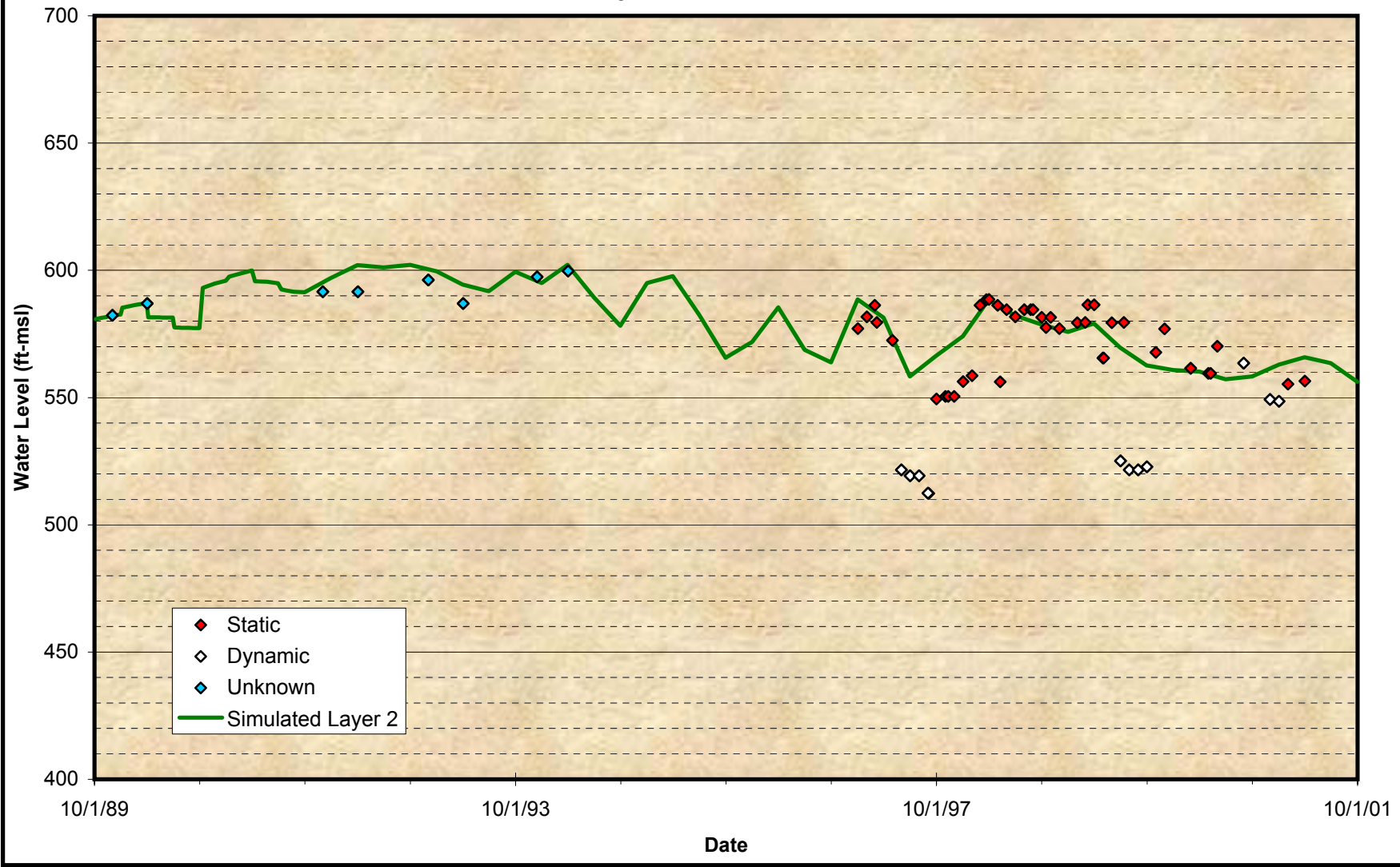
Figure A-15 Comparison of Groundwater Model Projected Time Histories at Wells for the Calibration Period City of Pomona – No. 11
