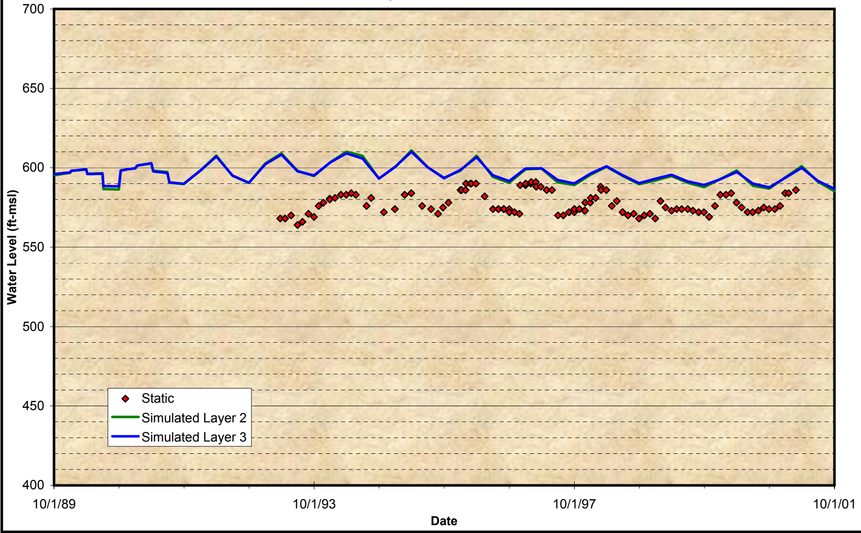
Figure A-19 Comparison of Groundwater Model Projected Time Histories at Wells for the Calibration Period City of Chino – No. 11
