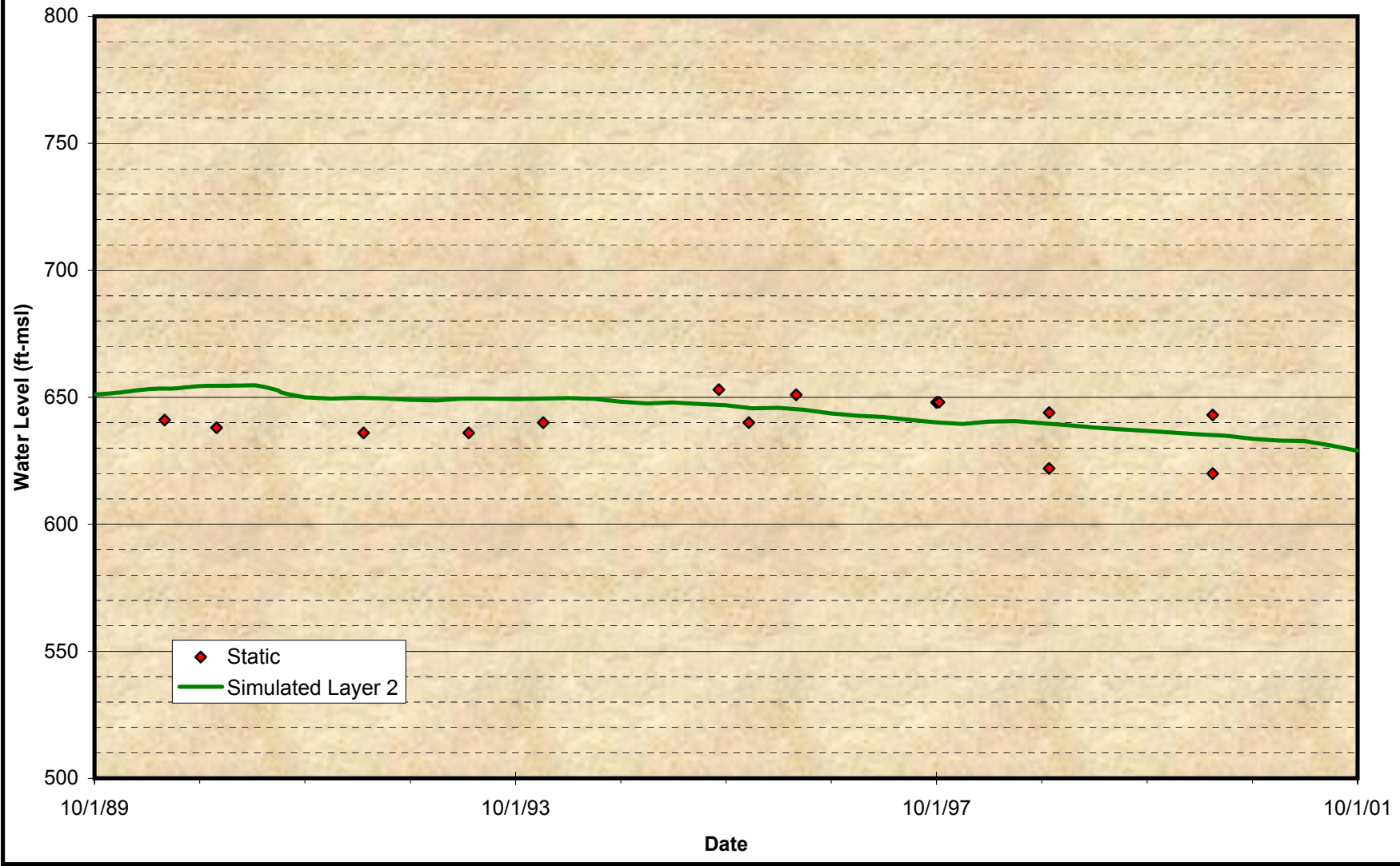
Figure A-13 Comparison of Groundwater Model Projected Time Histories at Wells for the Calibration Period City of Upland – No. 3
