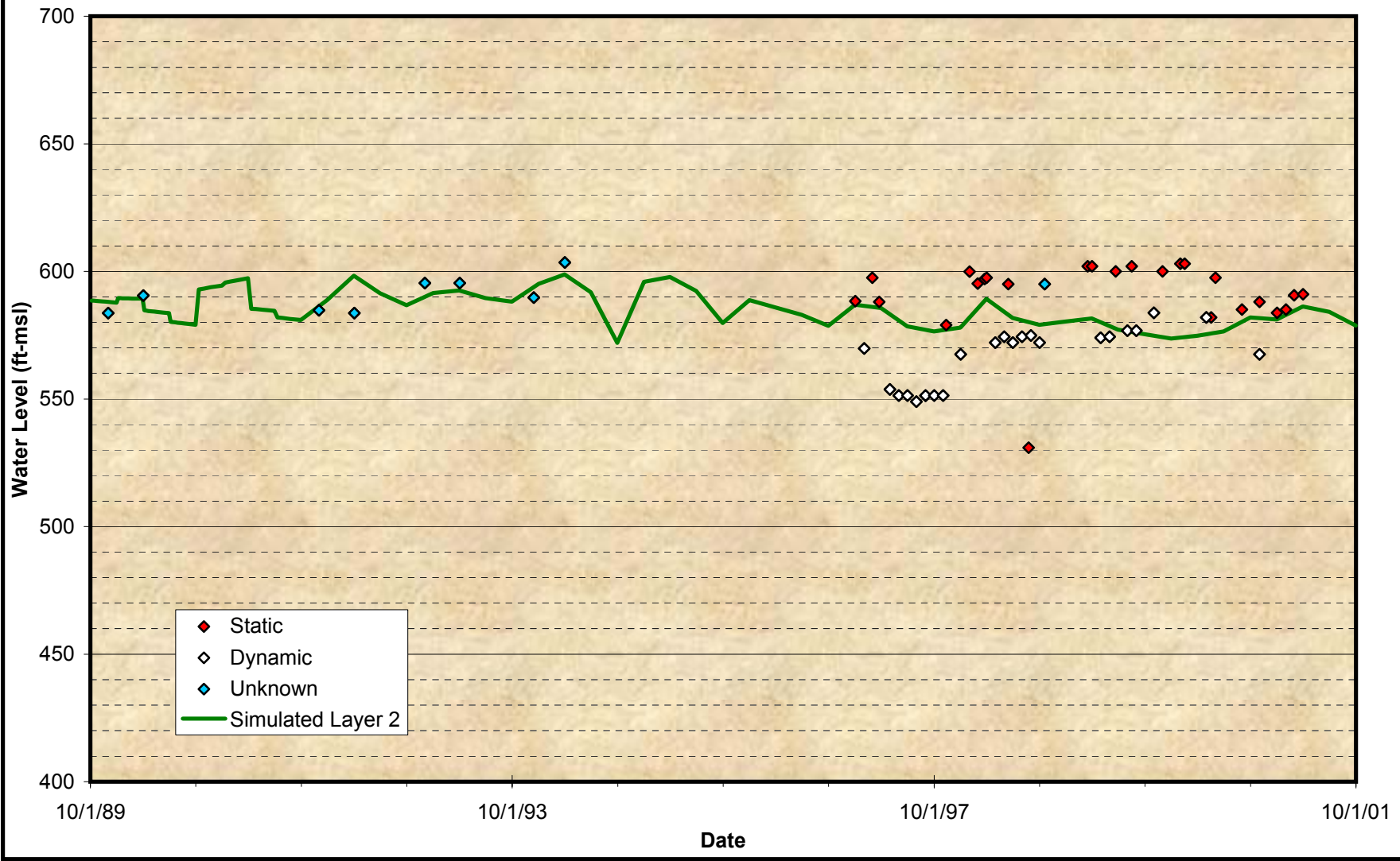
Figure A-18 Comparison of Groundwater Model Projected Time Histories at Wells for the Calibration Period City of Pomona – No. 29
