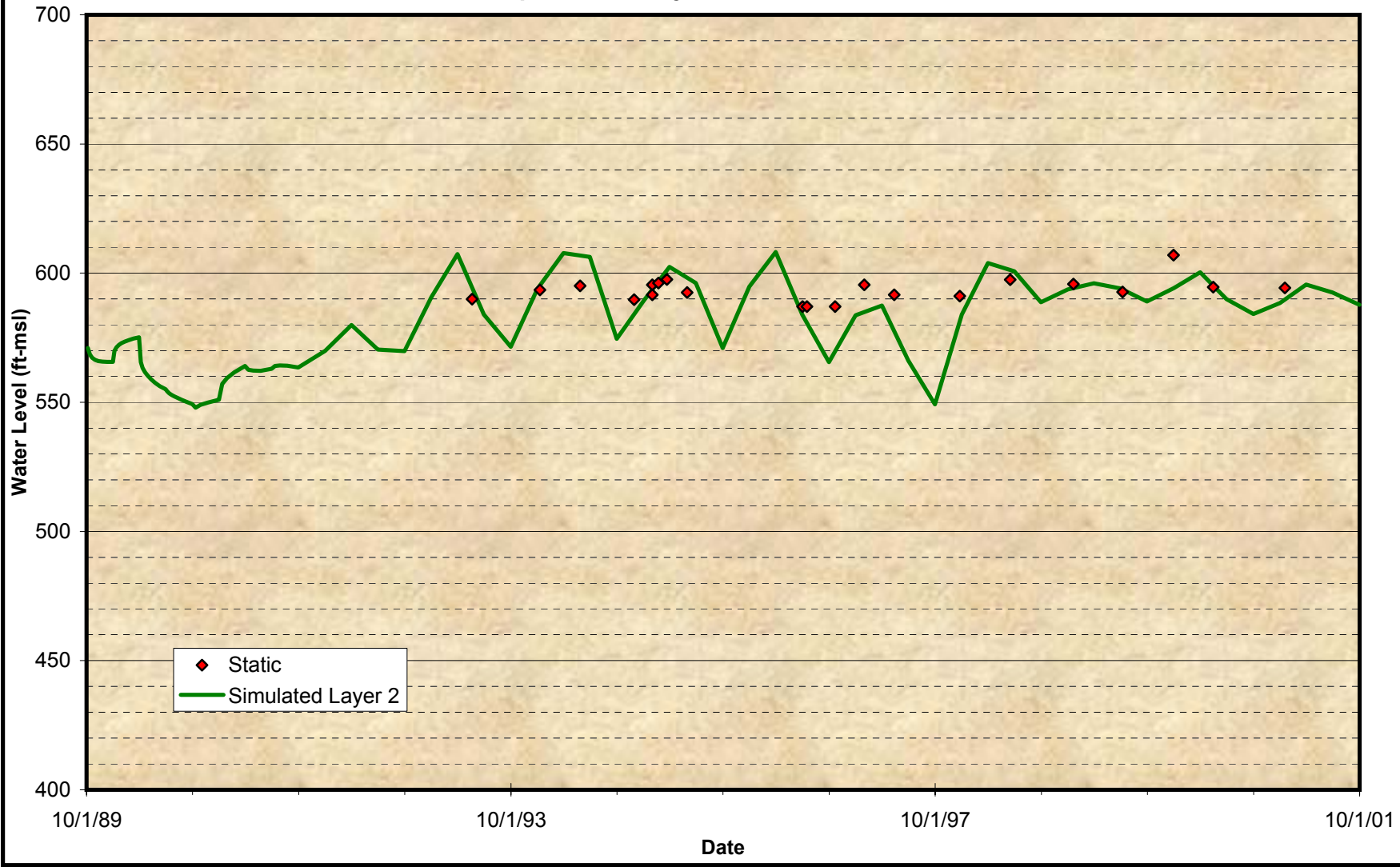
Figure A-30 Comparison of Groundwater Model Projected Time Histories at Wells for the Calibration Period Jurupa Community Services District – No. 16
