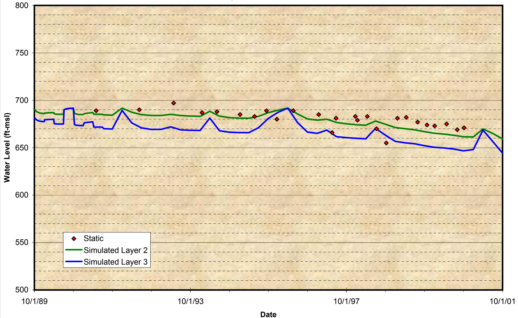
Figure A-9 Comparison of Groundwater Model Projected Time Histories at Wells for the Calibration Period City of Ontario – No. 31
