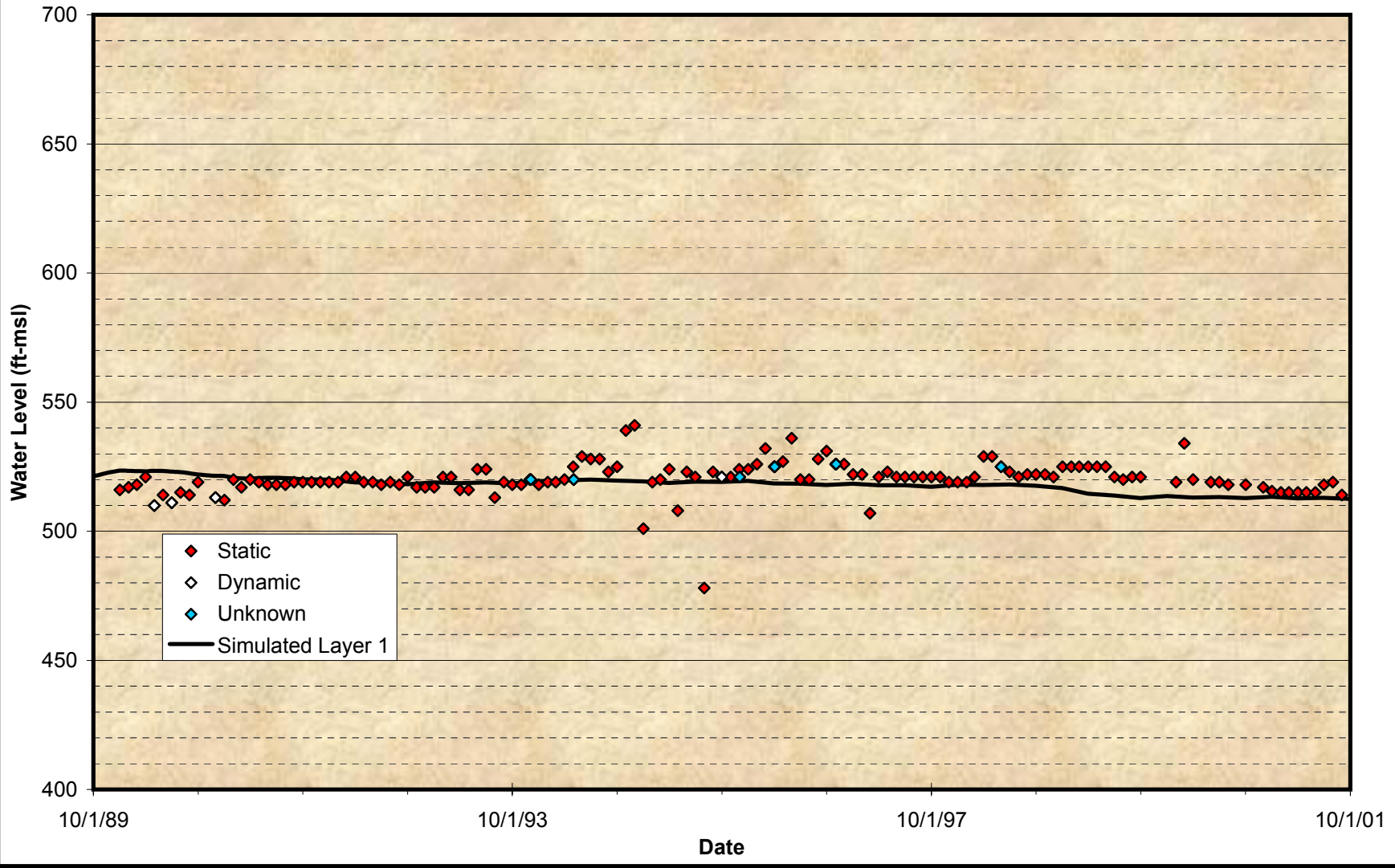
Figure A-45 Comparison of Groundwater Model Projected Time Histories at Wells for the Calibration Period City of Corona – No. 12
