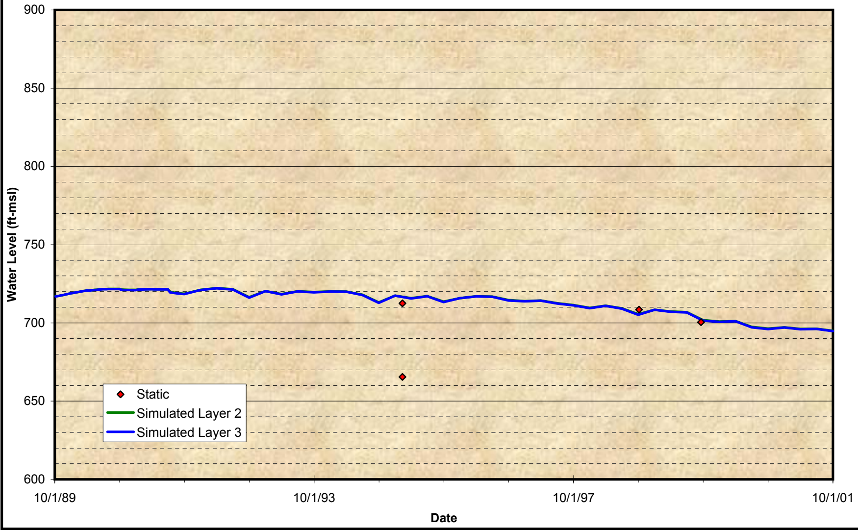
Figure A-8 Comparison of Groundwater Model Projected Time Histories at Wells for the Calibration Period Southern California Edison – Well C
