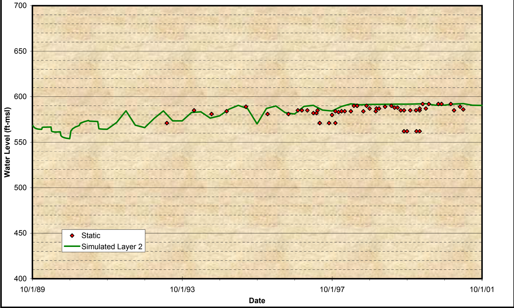
Figure A-31 Comparison of Groundwater Model Projected Time Histories at Wells for the Calibration Period City of Norco – No. 11
