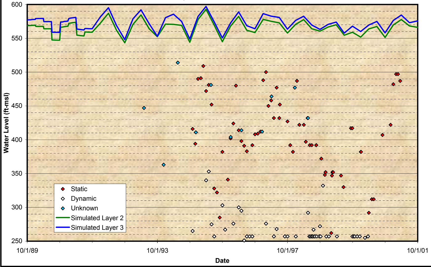
Figure A-28 Comparison of Groundwater Model Projected Time Histories at Wells for the Calibration Period City of Chino Hills – No. 15B
