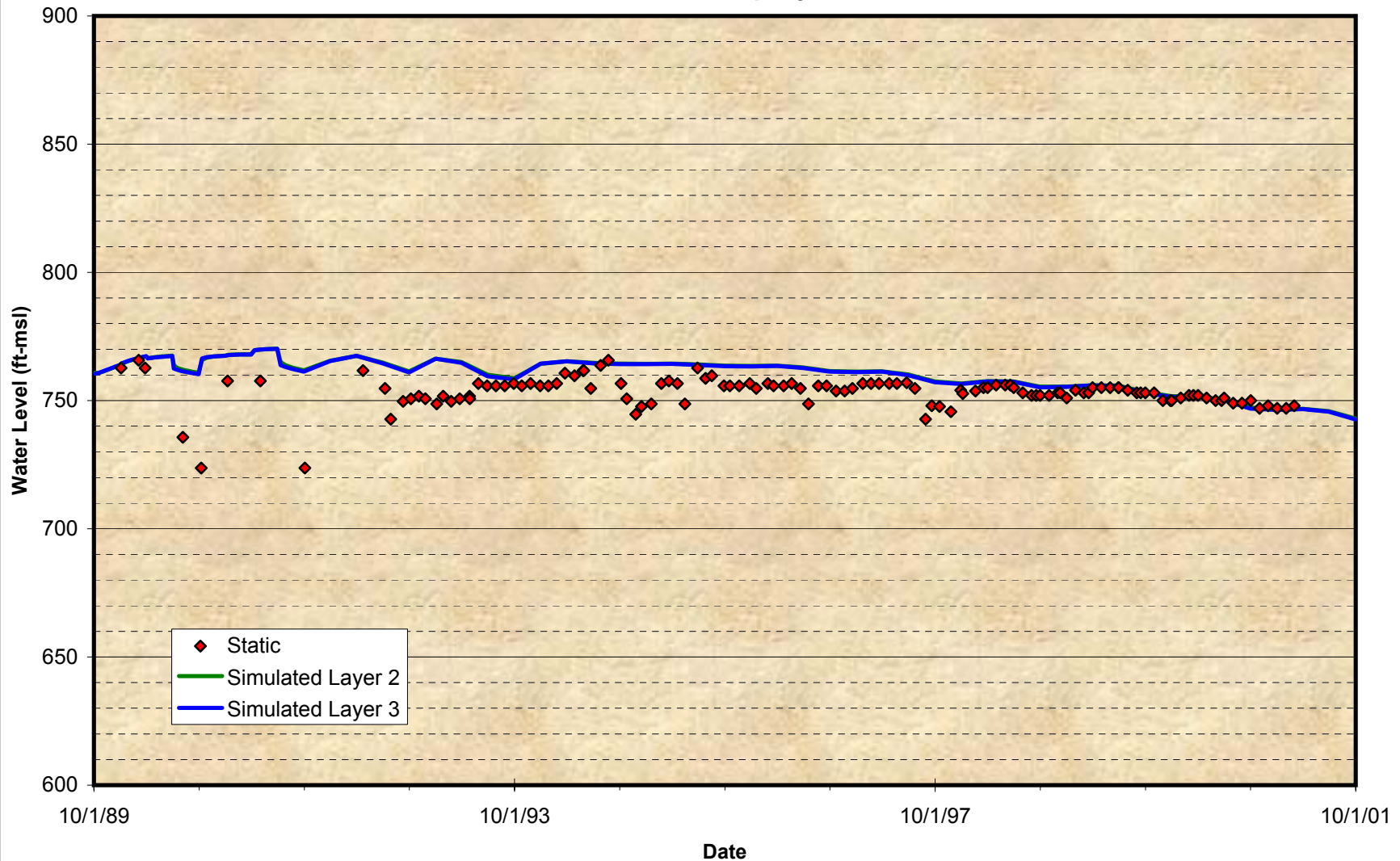
Figure A-5 Comparison of Groundwater Model Projected Time Histories at Wells for the Calibration Period Fontana Water Company – No. F3A
