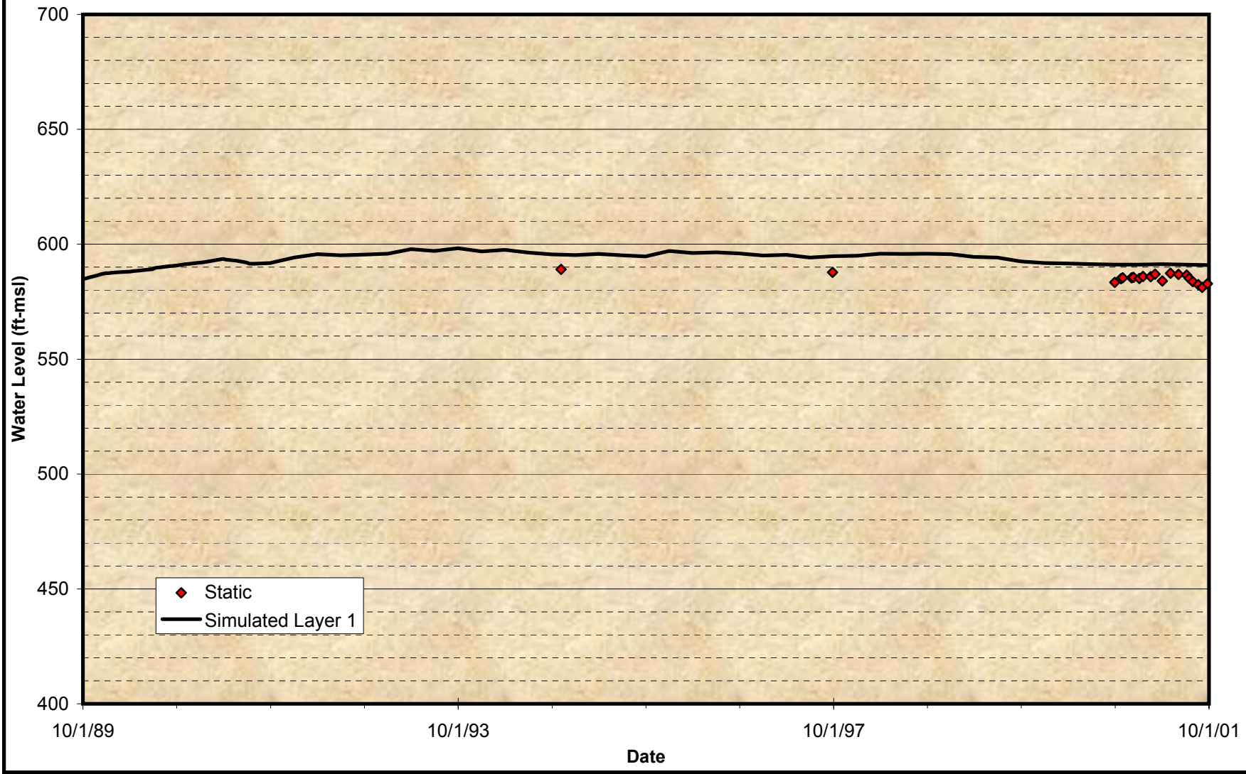
Figure A-32 Comparison of Groundwater Model Projected Time Histories at Wells for the Calibration Period Parente – ARC
