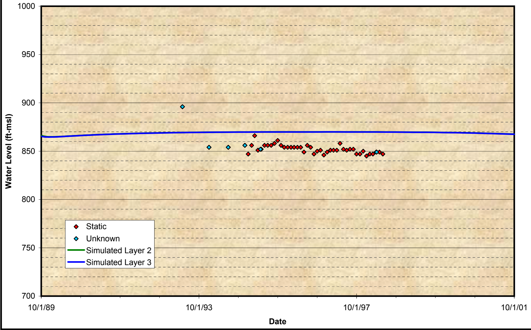
Figure A-1 Comparison of Groundwater Model Projected Time Histories at Wells for the Calibration Period City of Rialto – Chino No. 1
