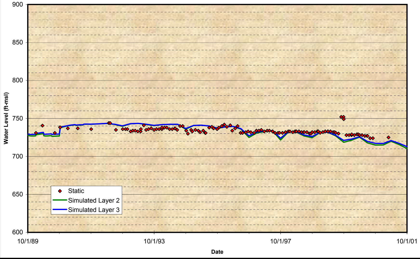
Figure A-6 Comparison of Groundwater Model Projected Time Histories at Wells for the Calibration Period Fontana Water Company – No. F21A
