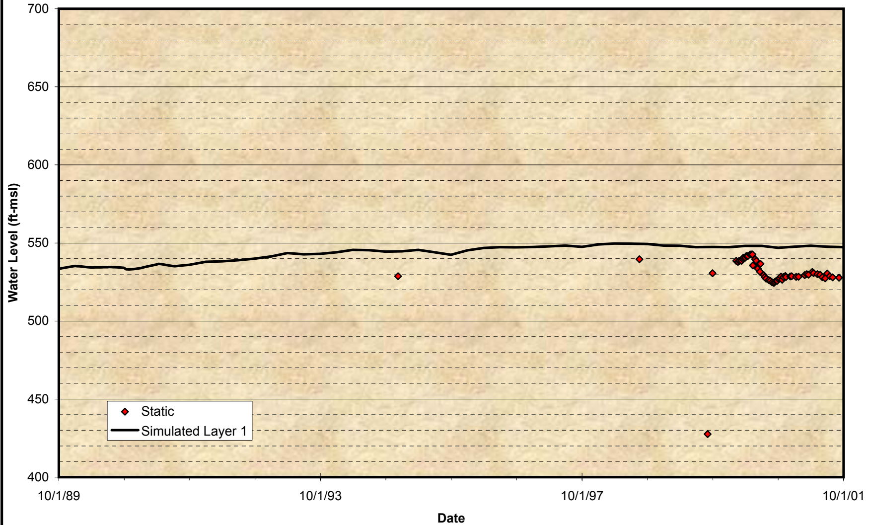
Figure A-40 Comparison of Groundwater Model Projected Time Histories at Wells for the Calibration Period Lekkerkerker – No. 2
