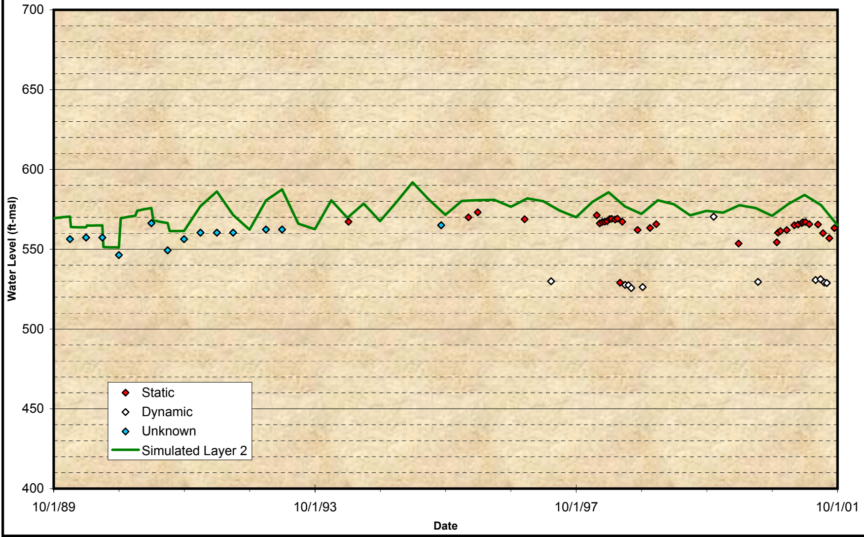
Figure A-22 Comparison of Groundwater Model Projected Time Histories at Wells for the Calibration Period CIM – No. 4
