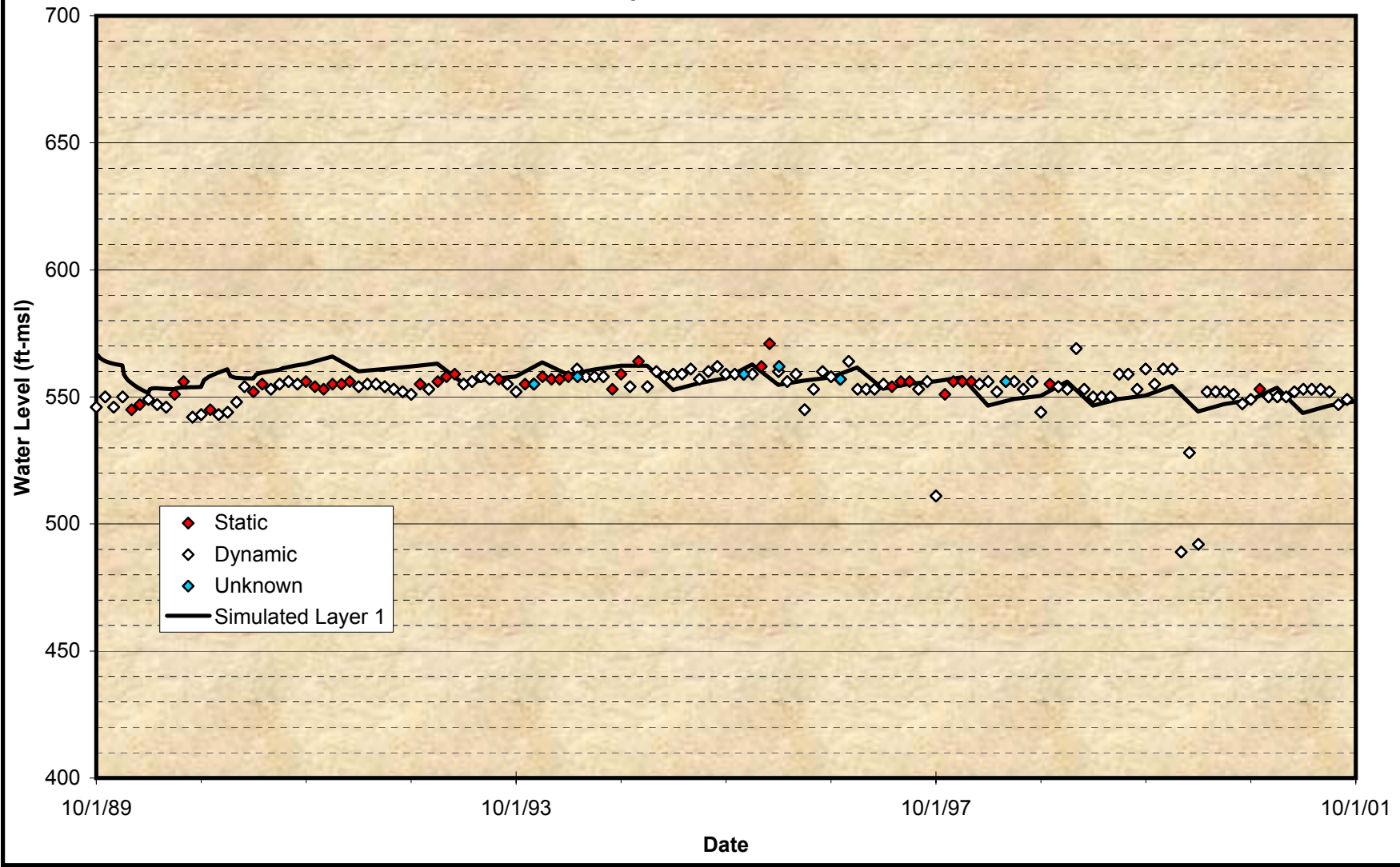
Figure A-42 Comparison of Groundwater Model Projected Time Histories at Wells for the Calibration Period City of Corona – No. 7
