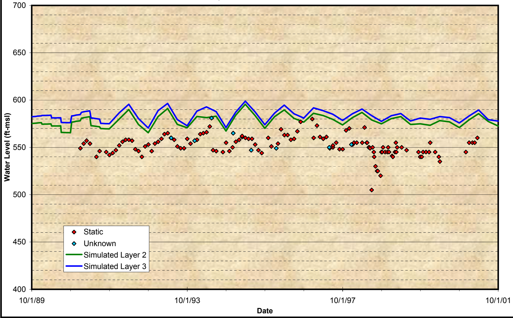
Figure A-25 Comparison of Groundwater Model Projected Time Histories at Wells for the Calibration Period City of Chino Hills – No. 18A
