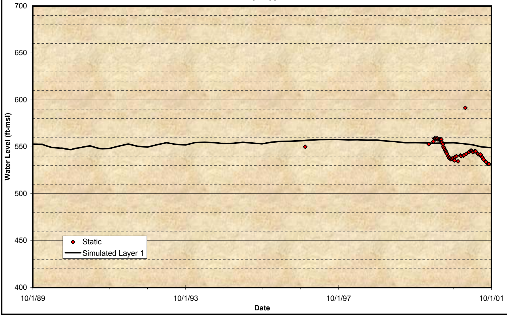
Figure A-37 Comparison of Groundwater Model Projected Time Histories at Wells for the Calibration Period DeVries
