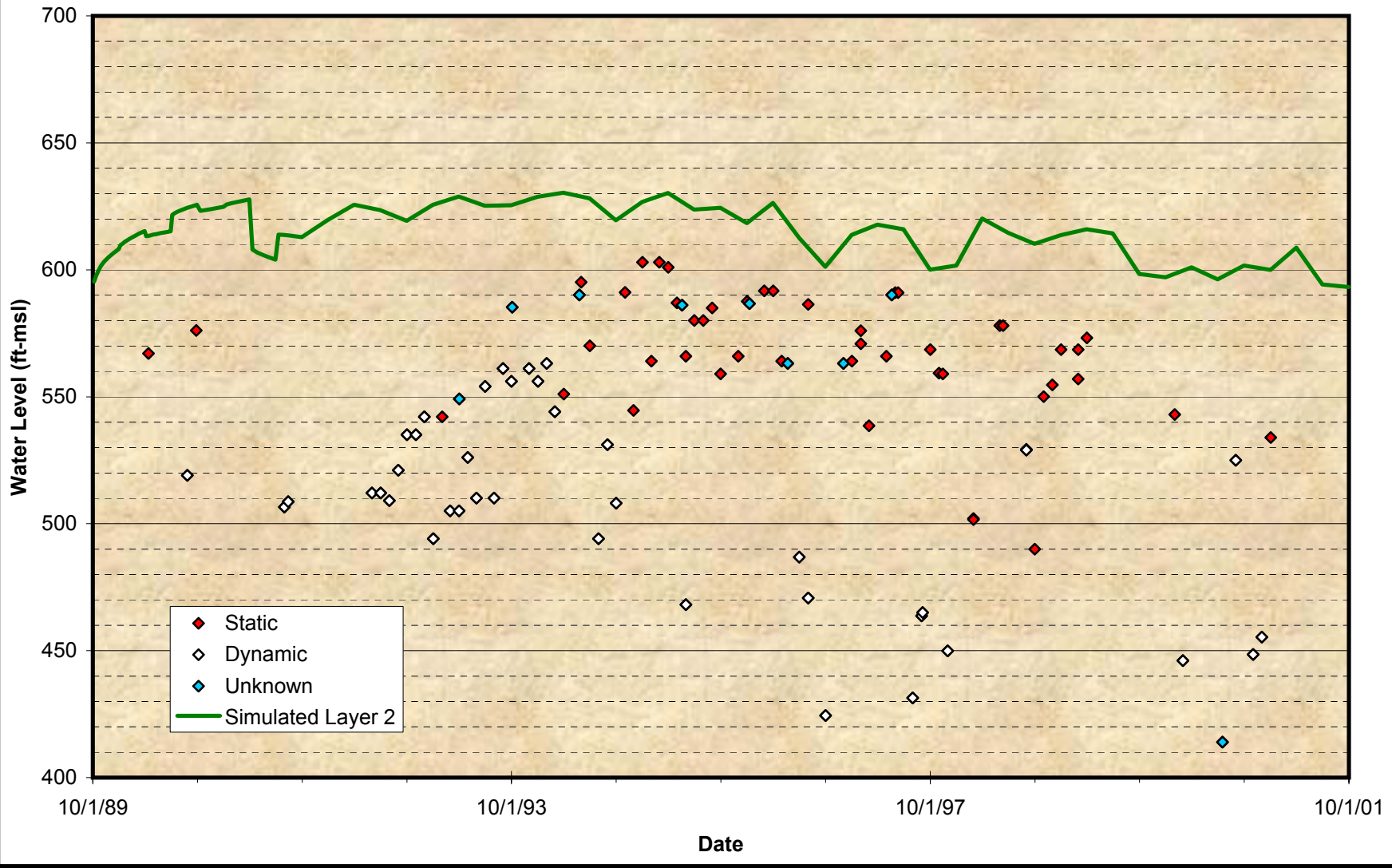
Figure A-14 Comparison of Groundwater Model Projected Time Histories at Wells for the Calibration Period Monte Vista Water District – No. 10
