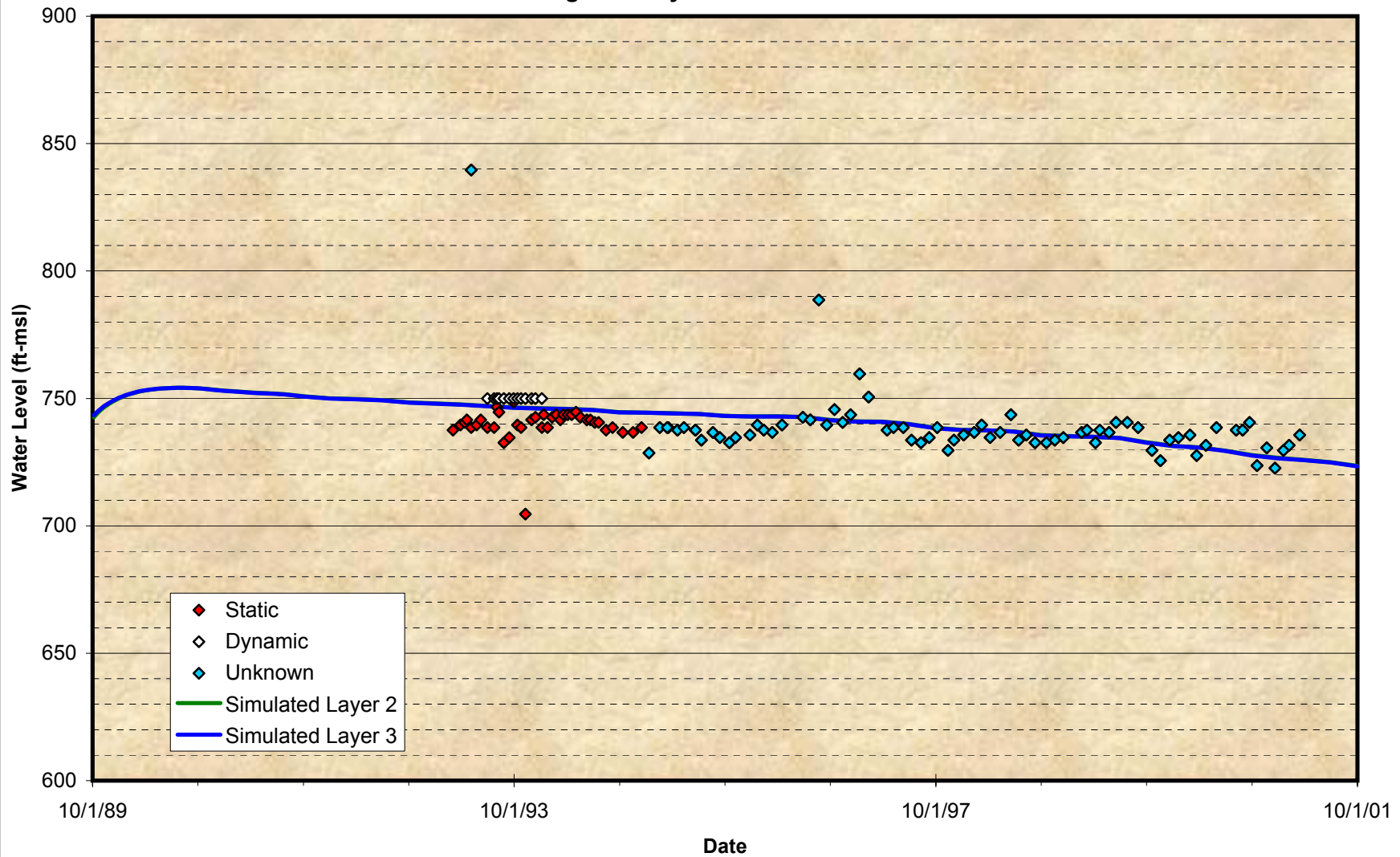
Figure A-7 Comparison of Groundwater Model Projected Time Histories at Wells for the Calibration Period Cucamonga County Water District – No. CB-35
