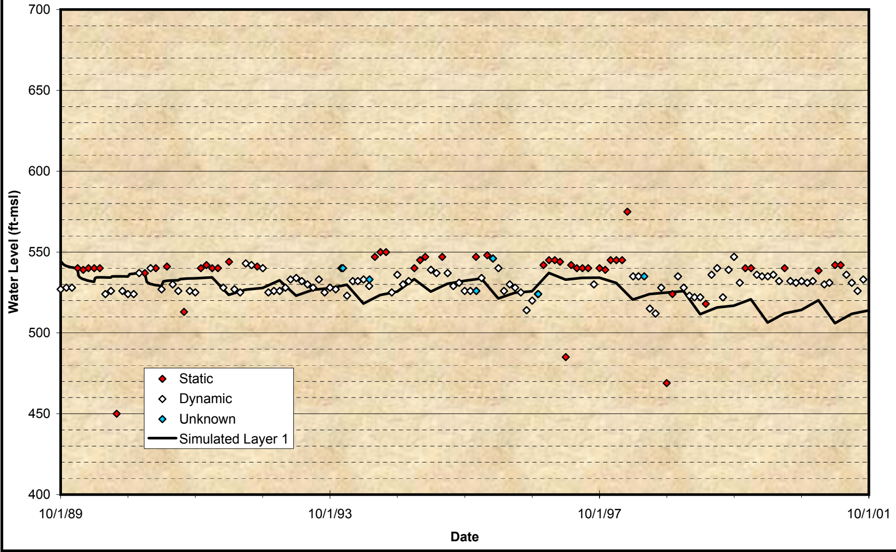
Figure A-44 Comparison of Groundwater Model Projected Time Histories at Wells for the Calibration Period City of Corona – No. 15
