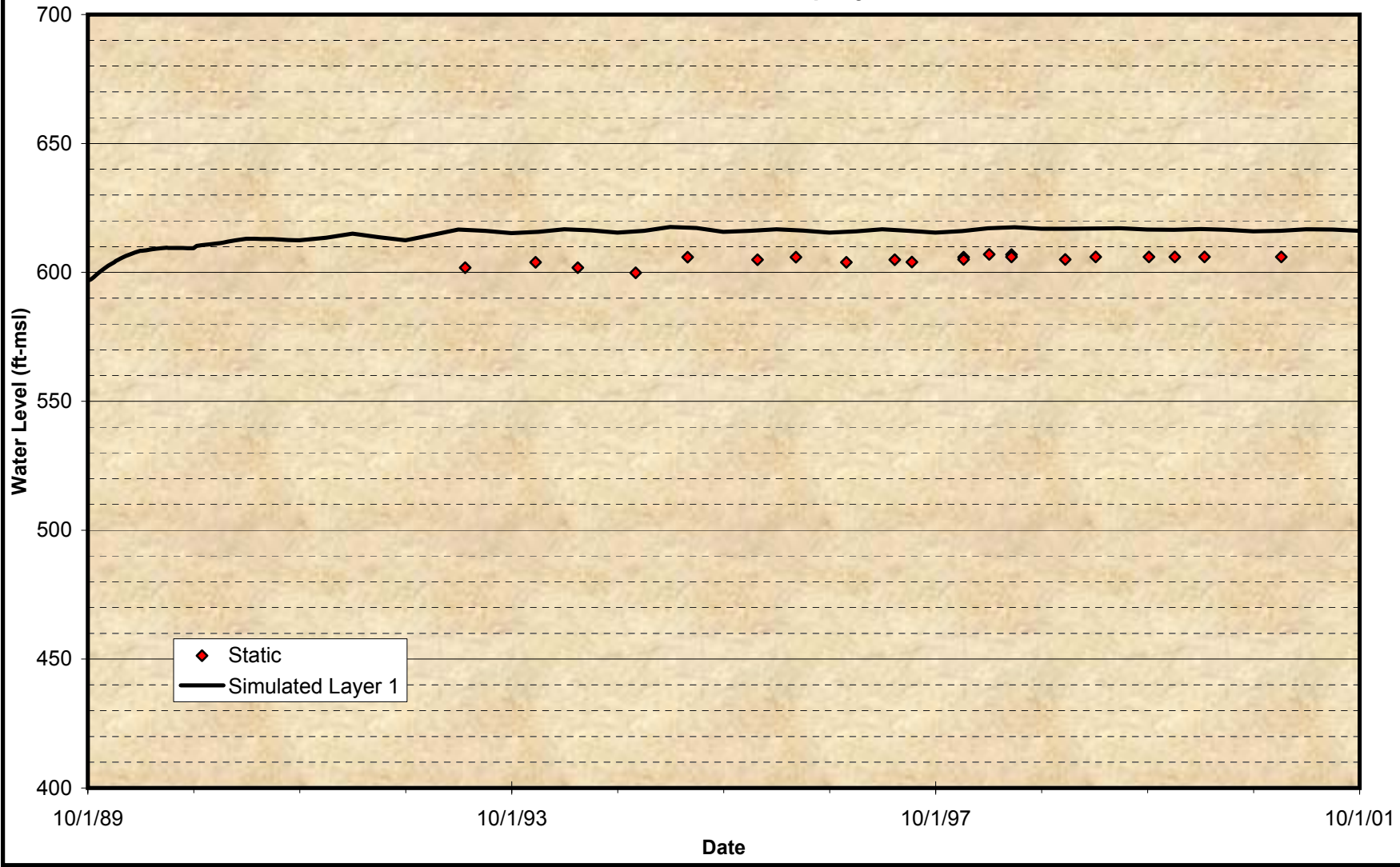
Figure A-29 Comparison of Groundwater Model Projected Time Histories at Wells for the Calibration Period Santa Ana River Water Company – No. 7
