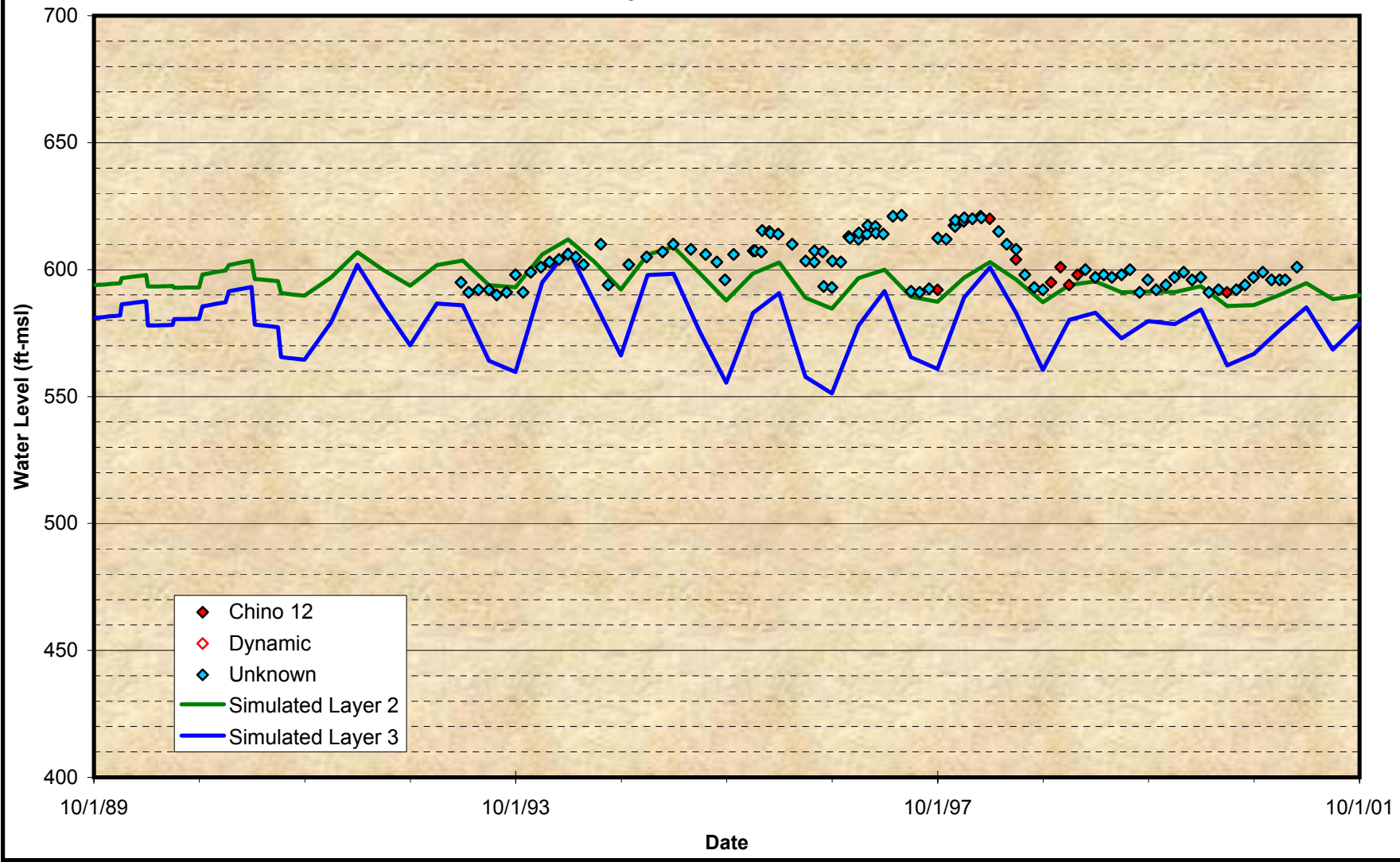
Figure A-16 Comparison of Groundwater Model Projected Time Histories at Wells for the Calibration Period City of Chino – No. 12
