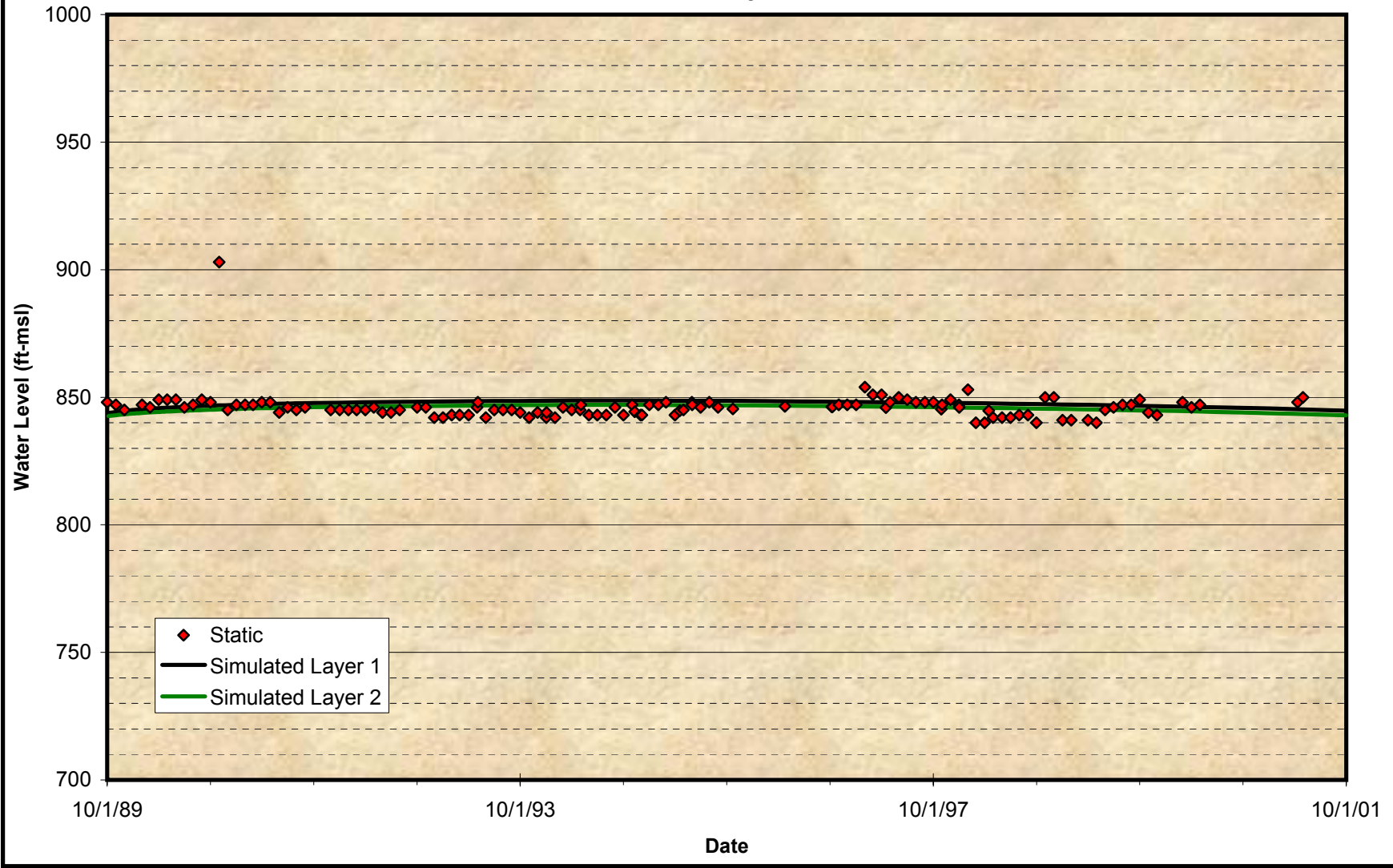
Figure A-2 Comparison of Groundwater Model Projected Time Histories at Wells for the Calibration Period West San Bernardino County Water District – No. 27
