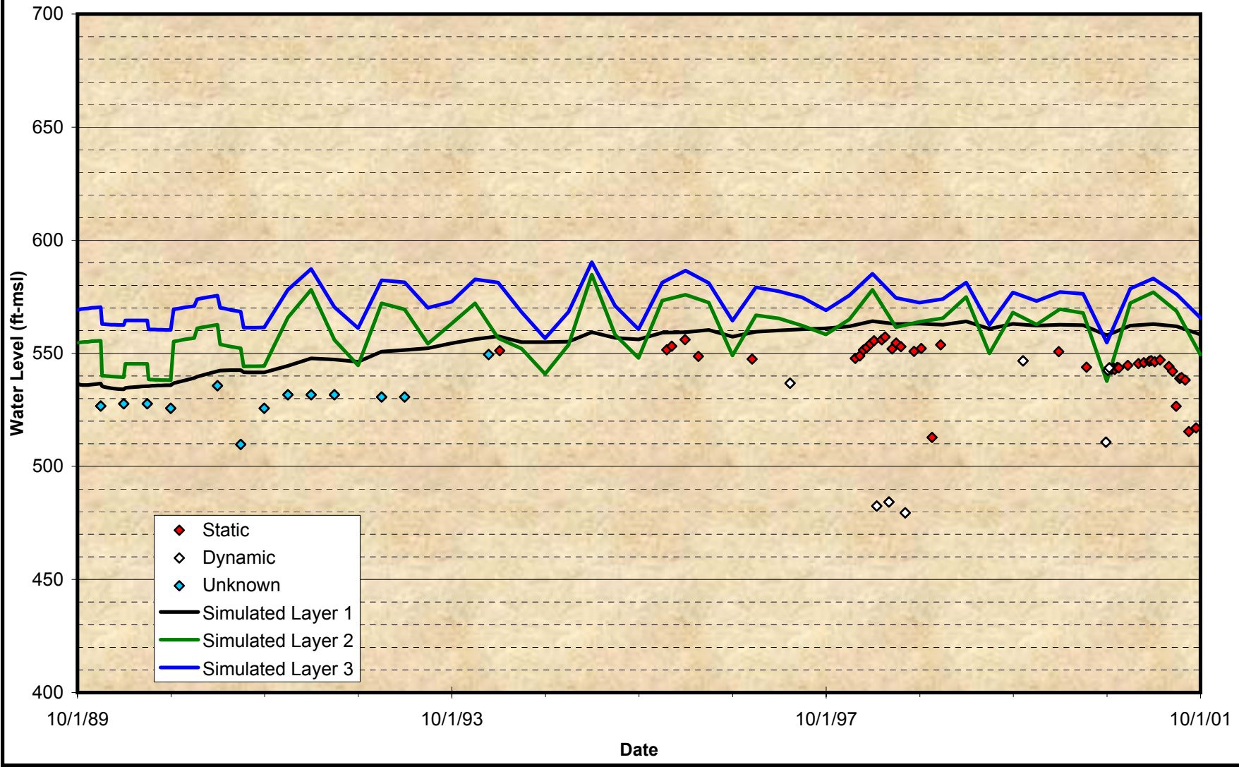
Figure A-23 Comparison of Groundwater Model Projected Time Histories at Wells for the Calibration Period CIM – No. 13
