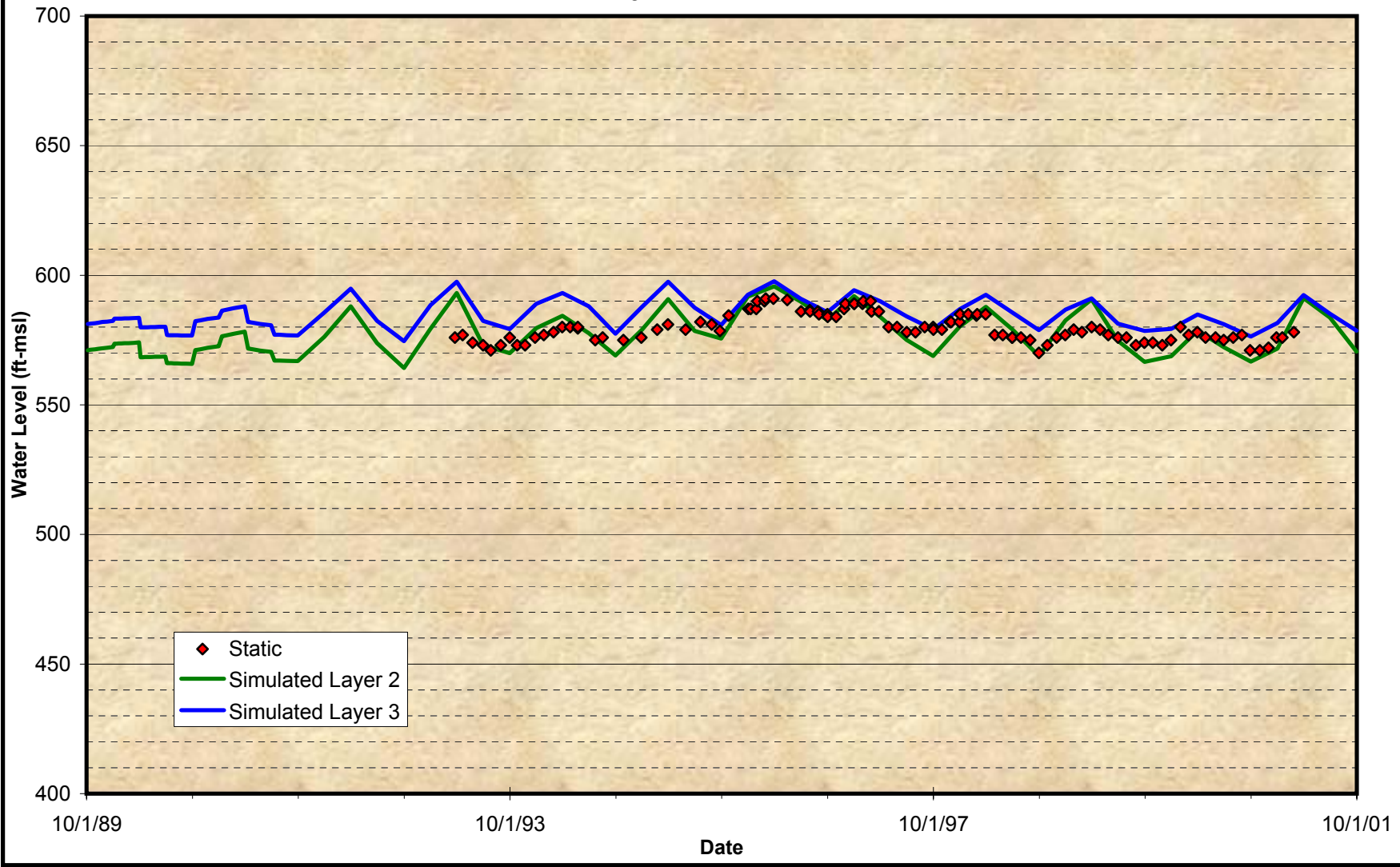
Figure A-20 Comparison of Groundwater Model Projected Time Histories at Wells for the Calibration Period City of Chino – No. 13
