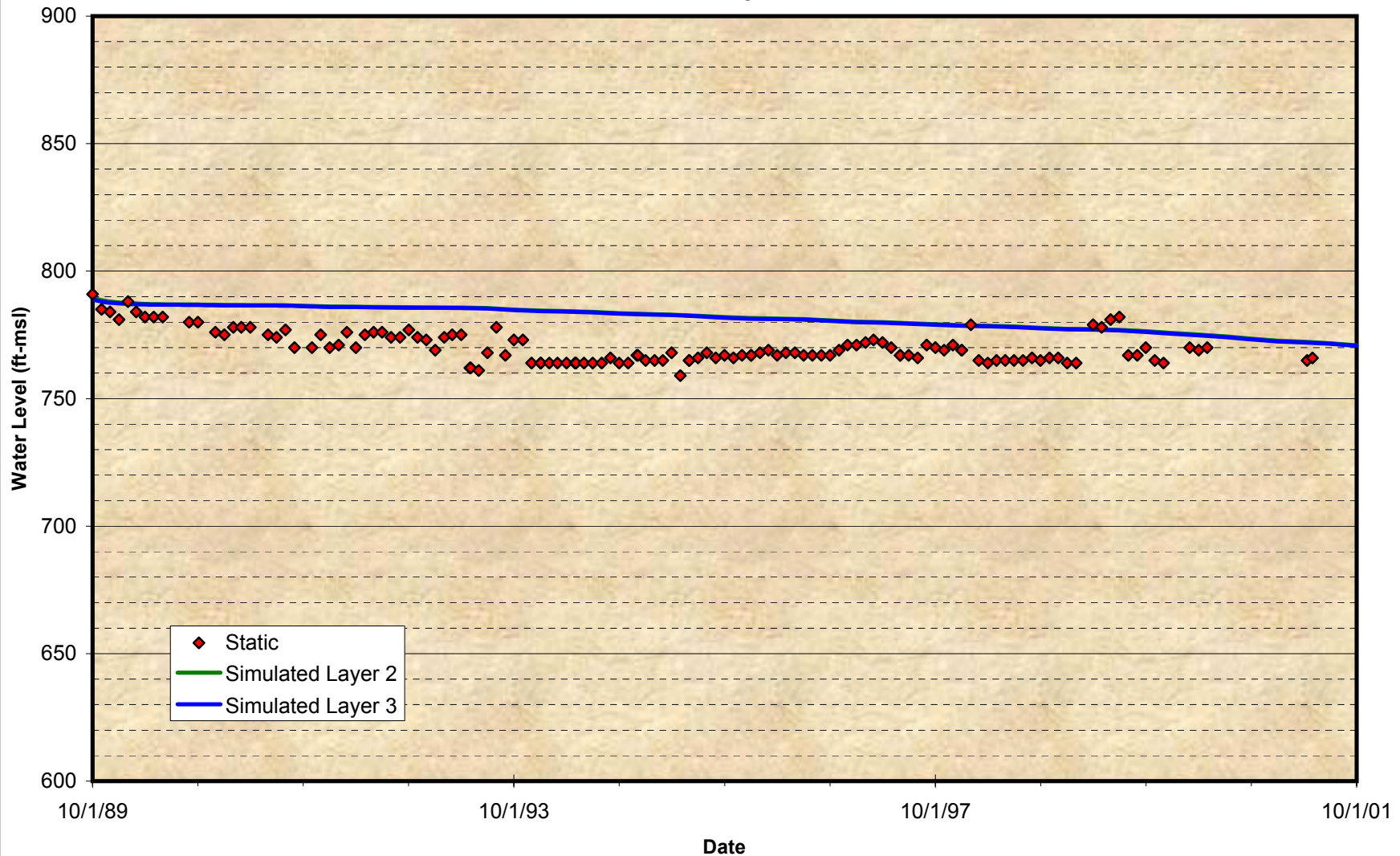
Figure A-3 Comparison of Groundwater Model Projected Time Histories at Wells for the Calibration Period West San Bernardino County Water District – No. 37
