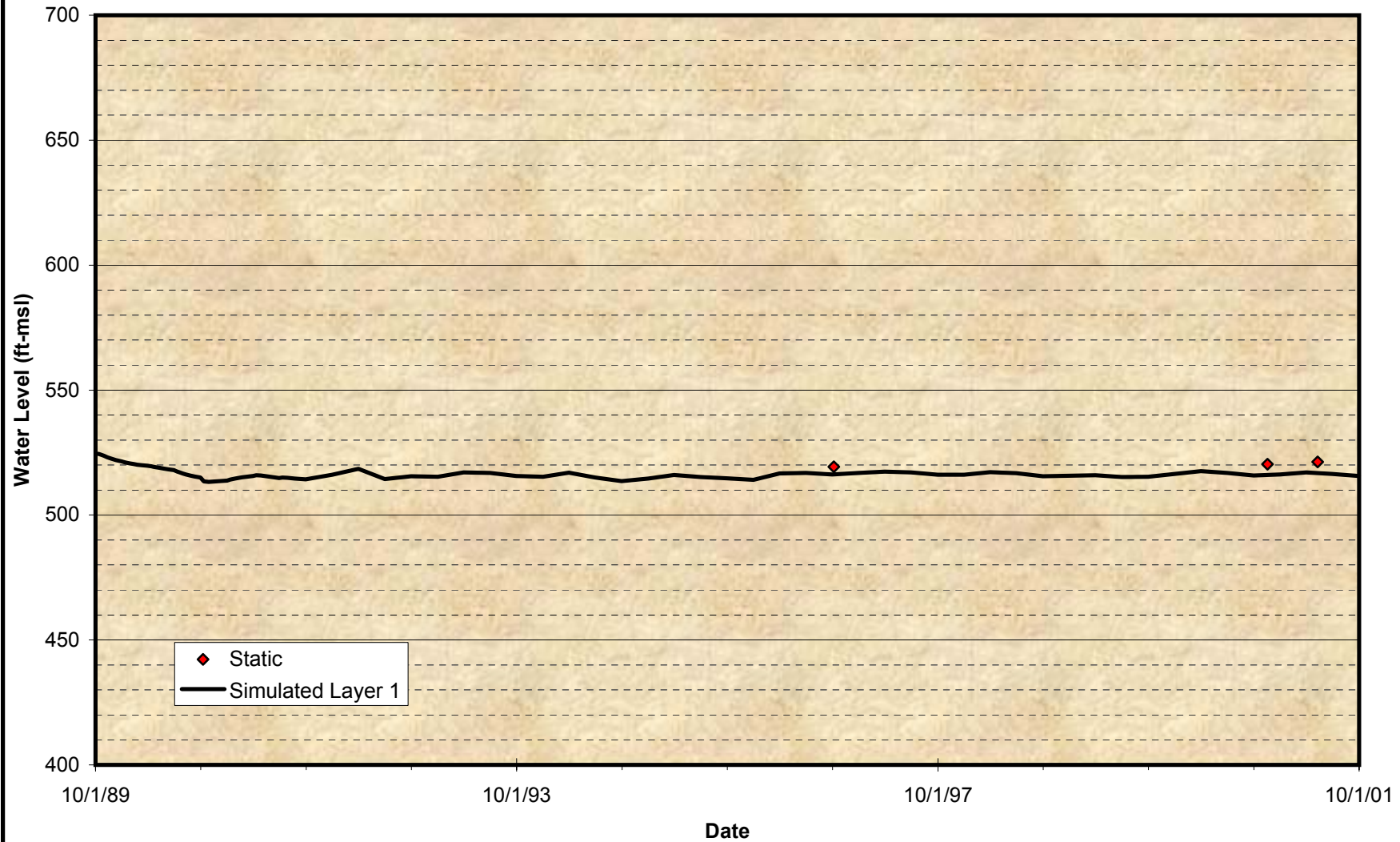
Figure A-41 Comparison of Groundwater Model Projected Time Histories at Wells for the Calibration Period Tollerup
