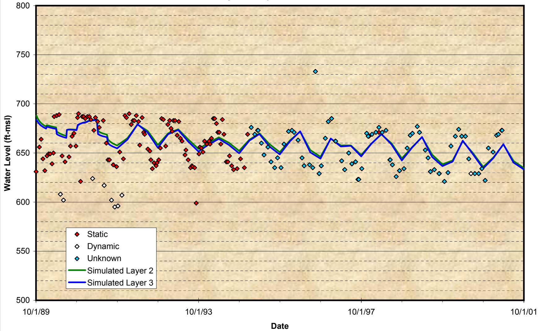
Figure A-10 Comparison of Groundwater Model Projected Time Histories at Wells for the Calibration Period Cucamonga County Water District – No. 30
