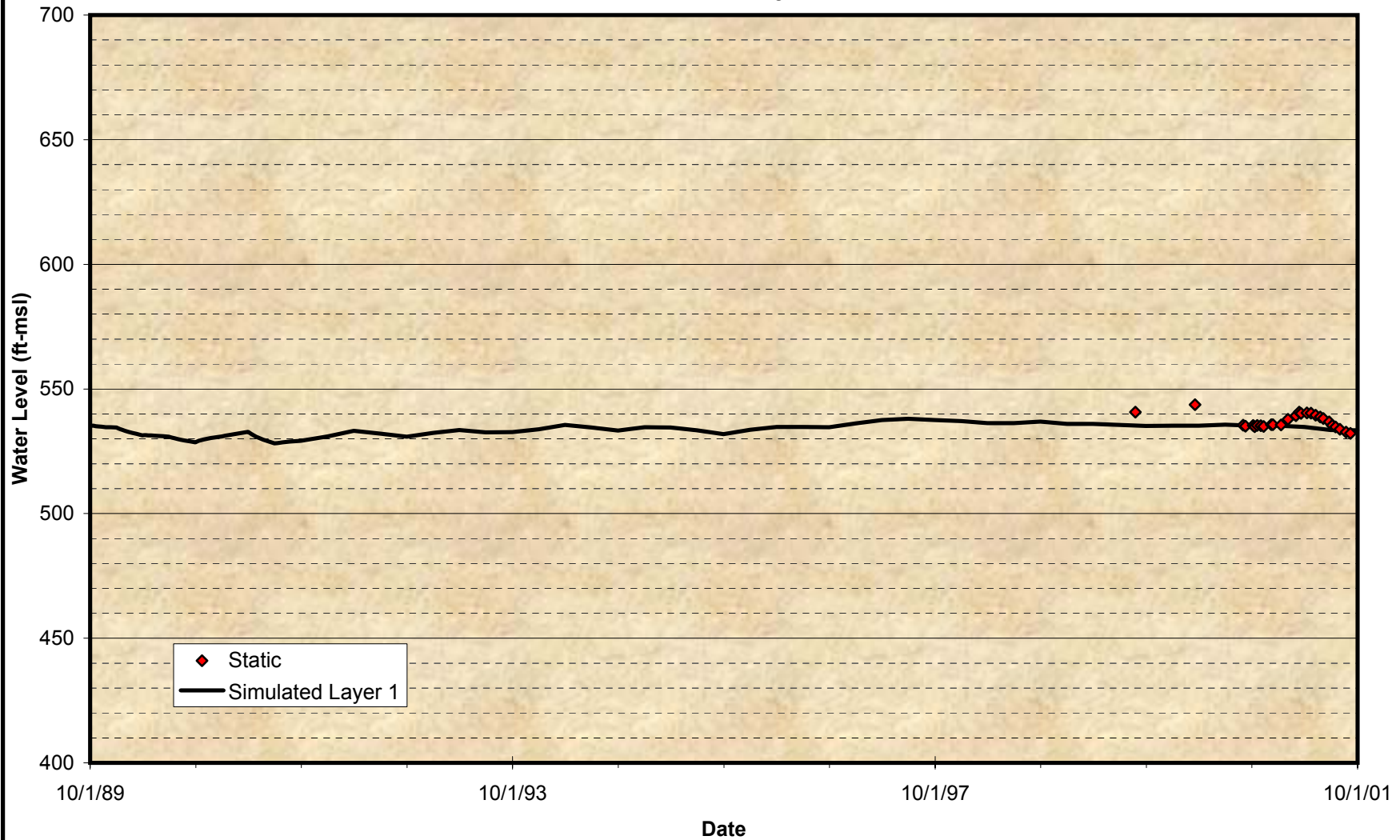
Figure A-39 Comparison of Groundwater Model Projected Time Histories at Wells for the Calibration Period Barthelemy
