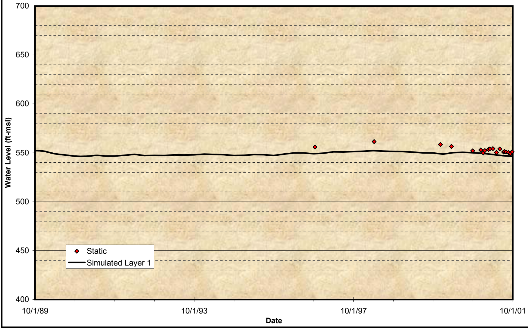
Figure A-34 Comparison of Groundwater Model Projected Time Histories at Wells for the Calibration Period Cardoza – No. B9
