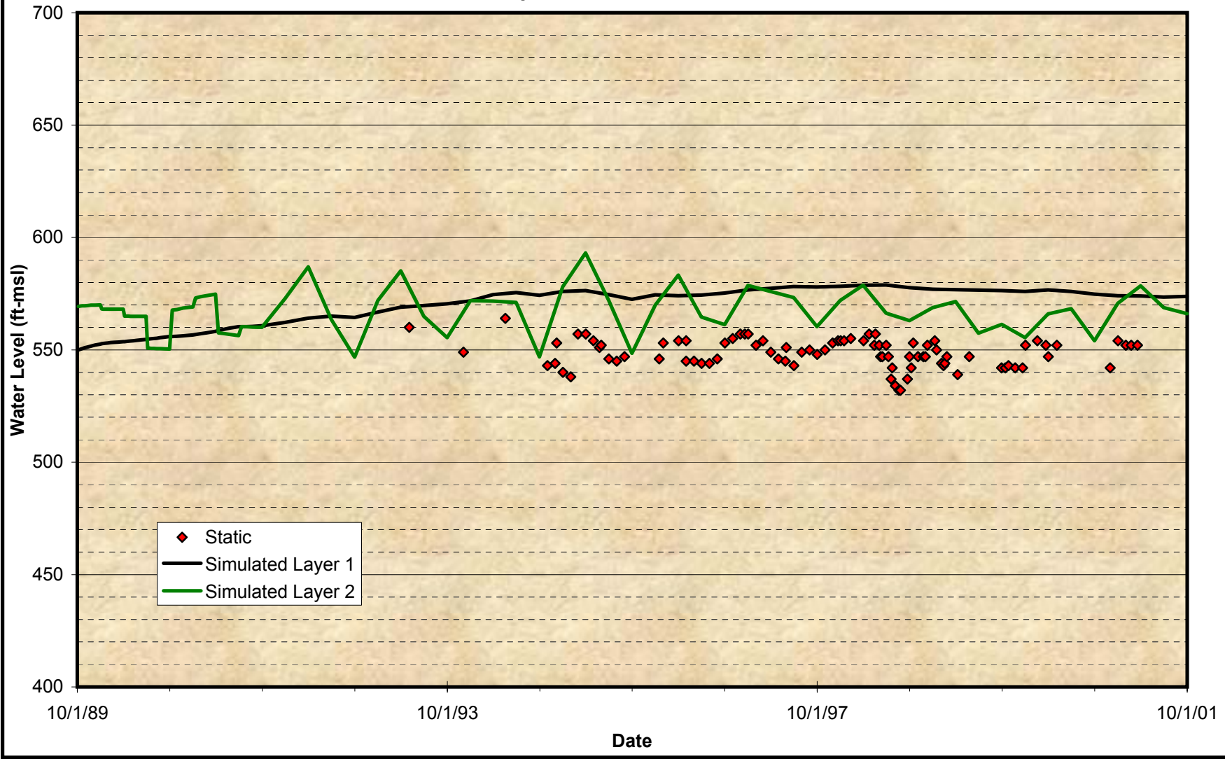
Figure A-27 Comparison of Groundwater Model Projected Time Histories at Wells for the Calibration Period City of Chino Hills – No. 15A
