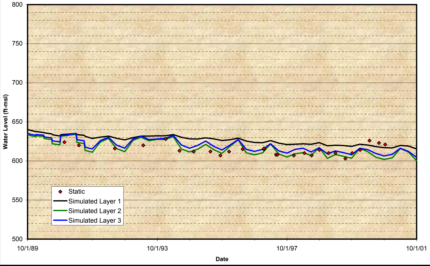
Figure A-12 Comparison of Groundwater Model Projected Time Histories at Wells for the Calibration Period City of Ontario – No. 17
