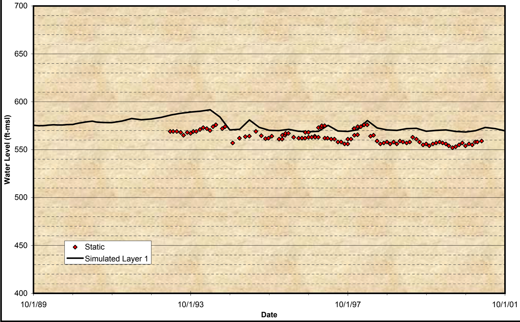
Figure A-21 Comparison of Groundwater Model Projected Time Histories at Wells for the Calibration Period City of Chino – No. 4
