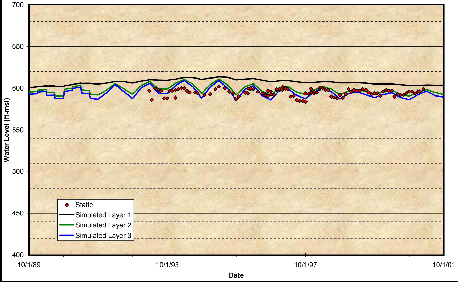
Figure A-17 Comparison of Groundwater Model Projected Time Histories at Wells for the Calibration Period City of Chino – No. 9
