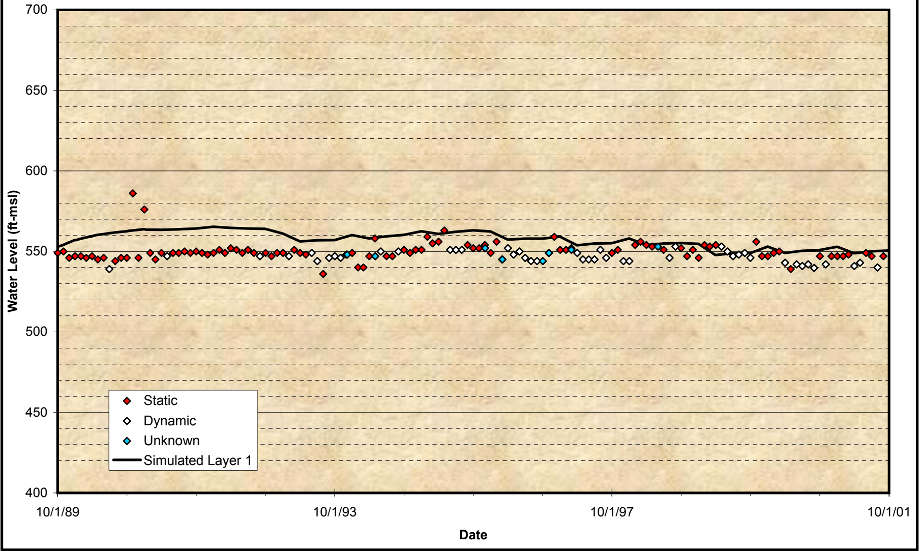
Figure A-43 Comparison of Groundwater Model Projected Time Histories at Wells for the Calibration Period City of Corona – No. 14
