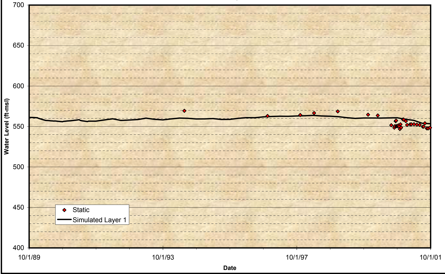
Figure A-36 Comparison of Groundwater Model Projected Time Histories at Wells for the Calibration Period Corona Dairy Ranch
