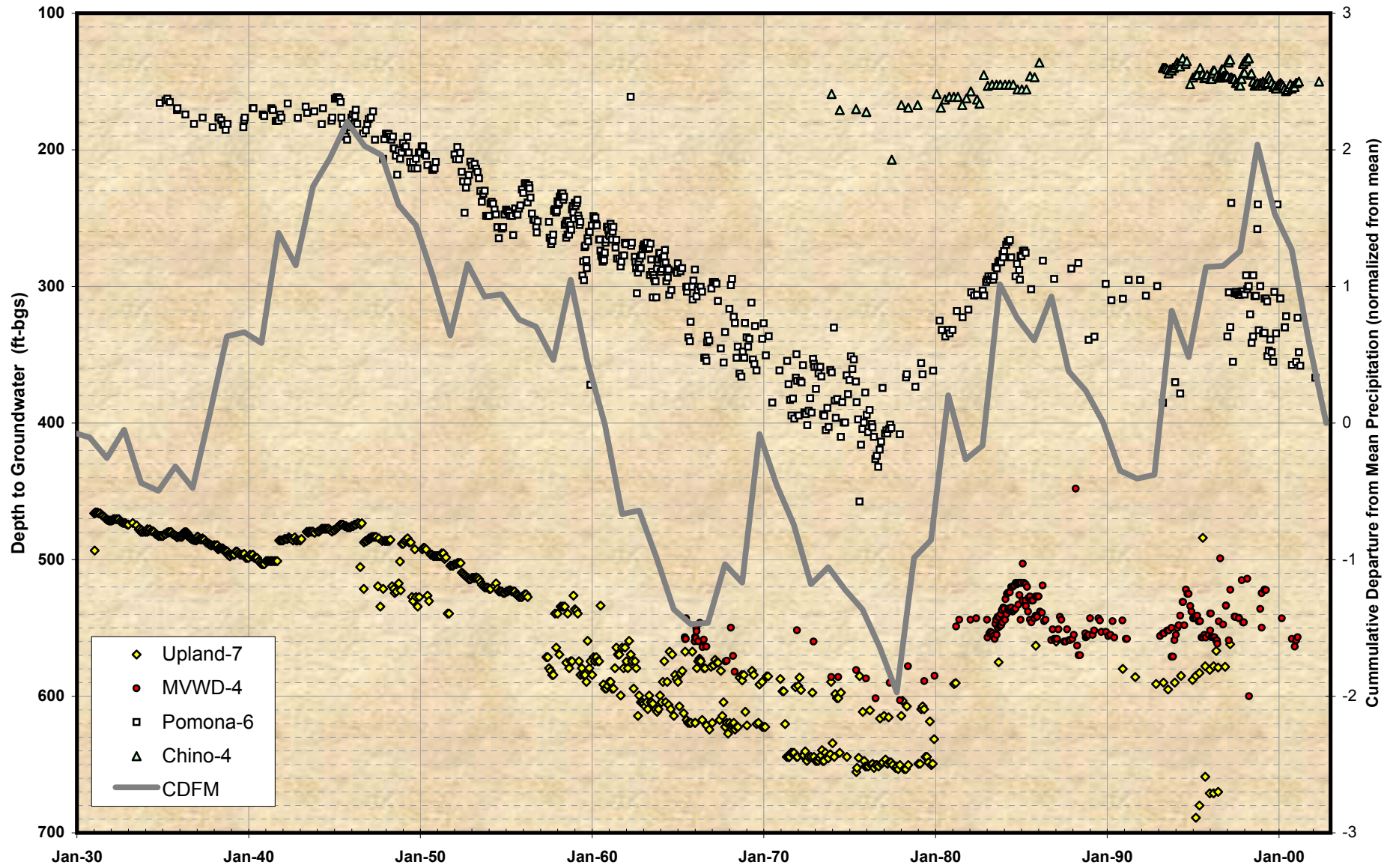
Figure 2-19 Water-Level Time Histories at Wells in Management Zone 1
