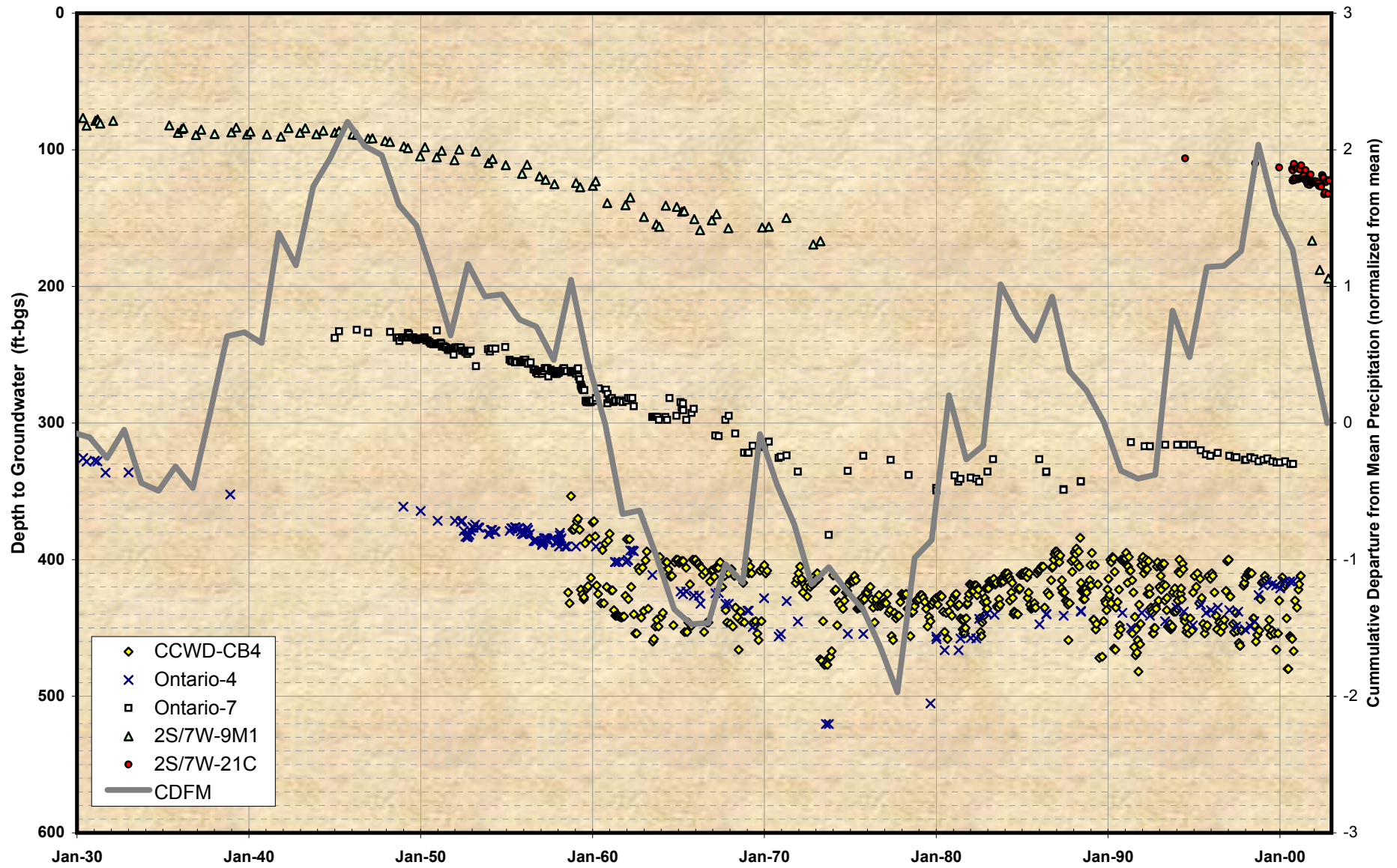
Figure 2-20 Water-Level Time Histories at Wells in Management Zone 2
