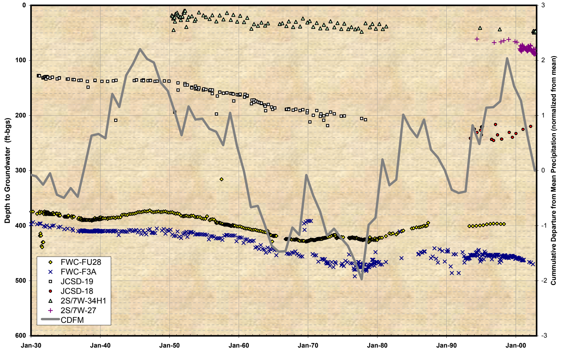
Figure 2-21 Water-Level Time Histories at Wells in Management Zone 3
