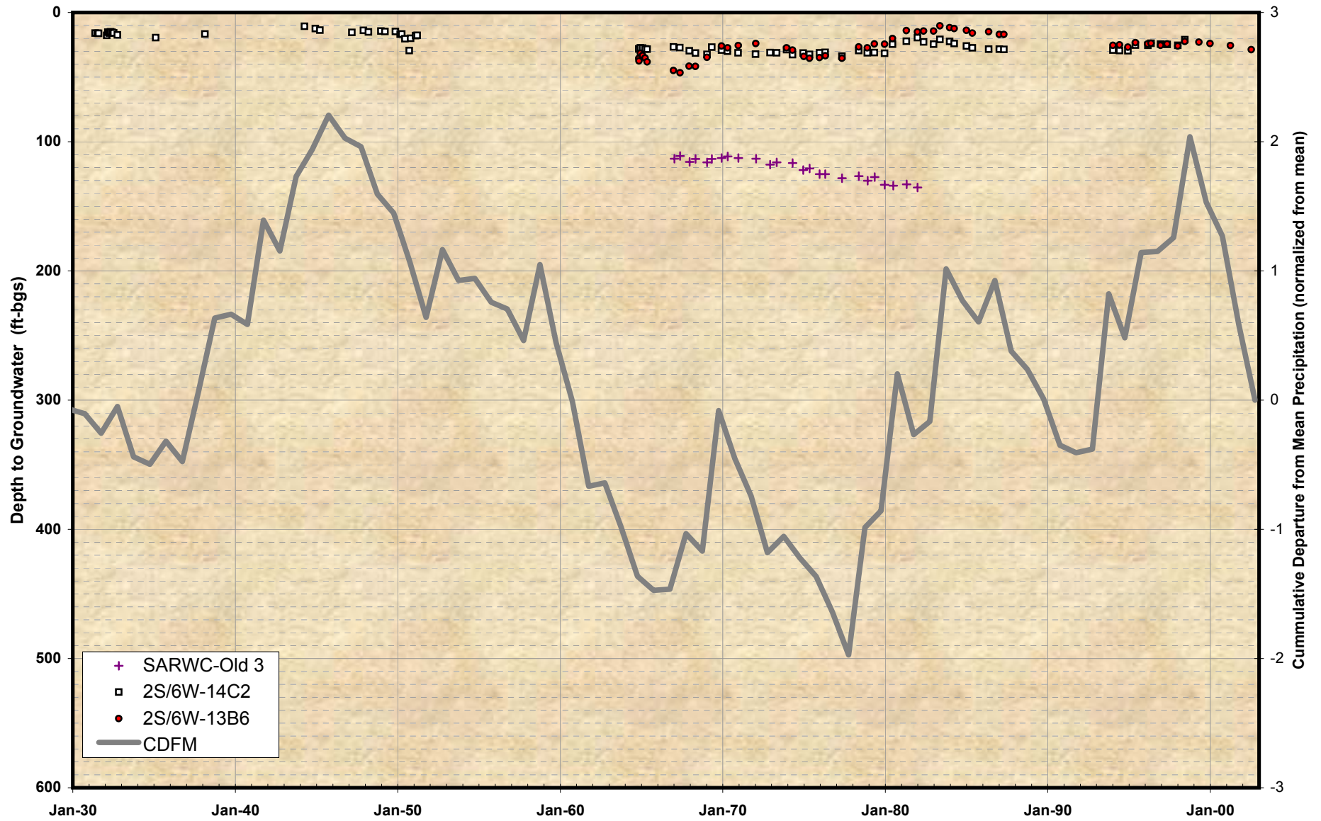
Figure 2-22 Water-Level Time Histories at Wells in Management Zone 4
