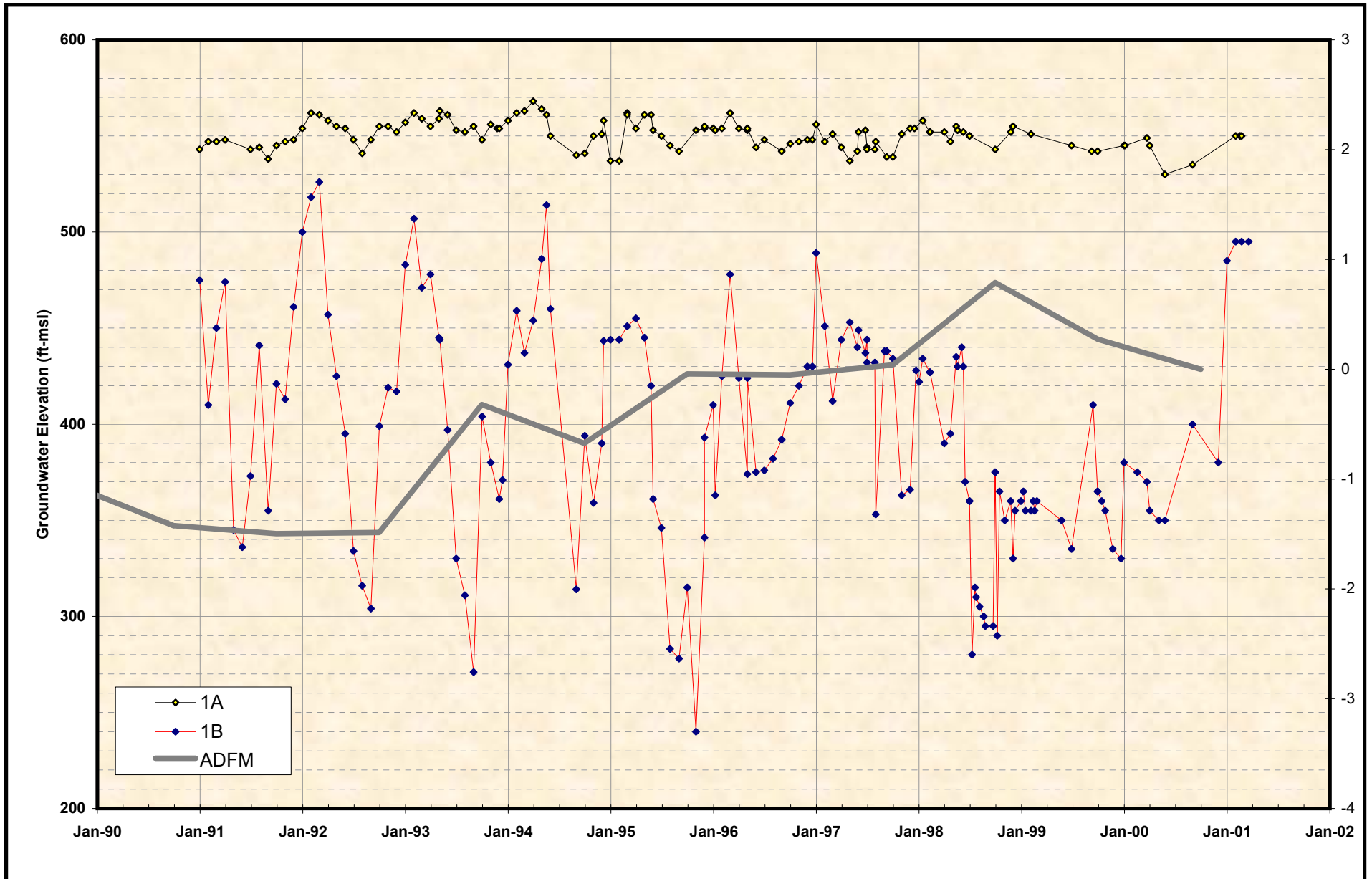
Figure 2-5 Water-Level Time Histories (Non-Pumping) at City of Chino Hills Wells 1A and 1B
