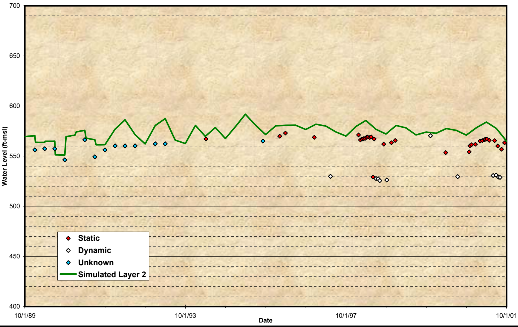
Figure 6-10 Comparison of Model Predicted Level and Observed Groundwater Level for CIM No. 4
