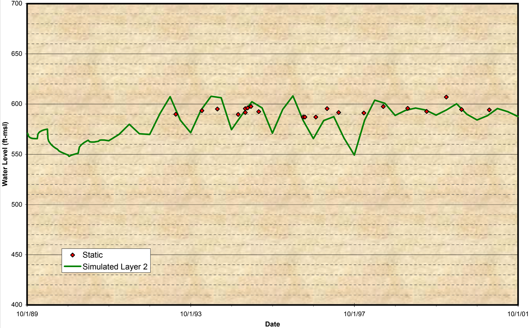
Figure 6-11 Comparison of Model Predicted Level and Observed Groundwater Level for JCSD No. 16
