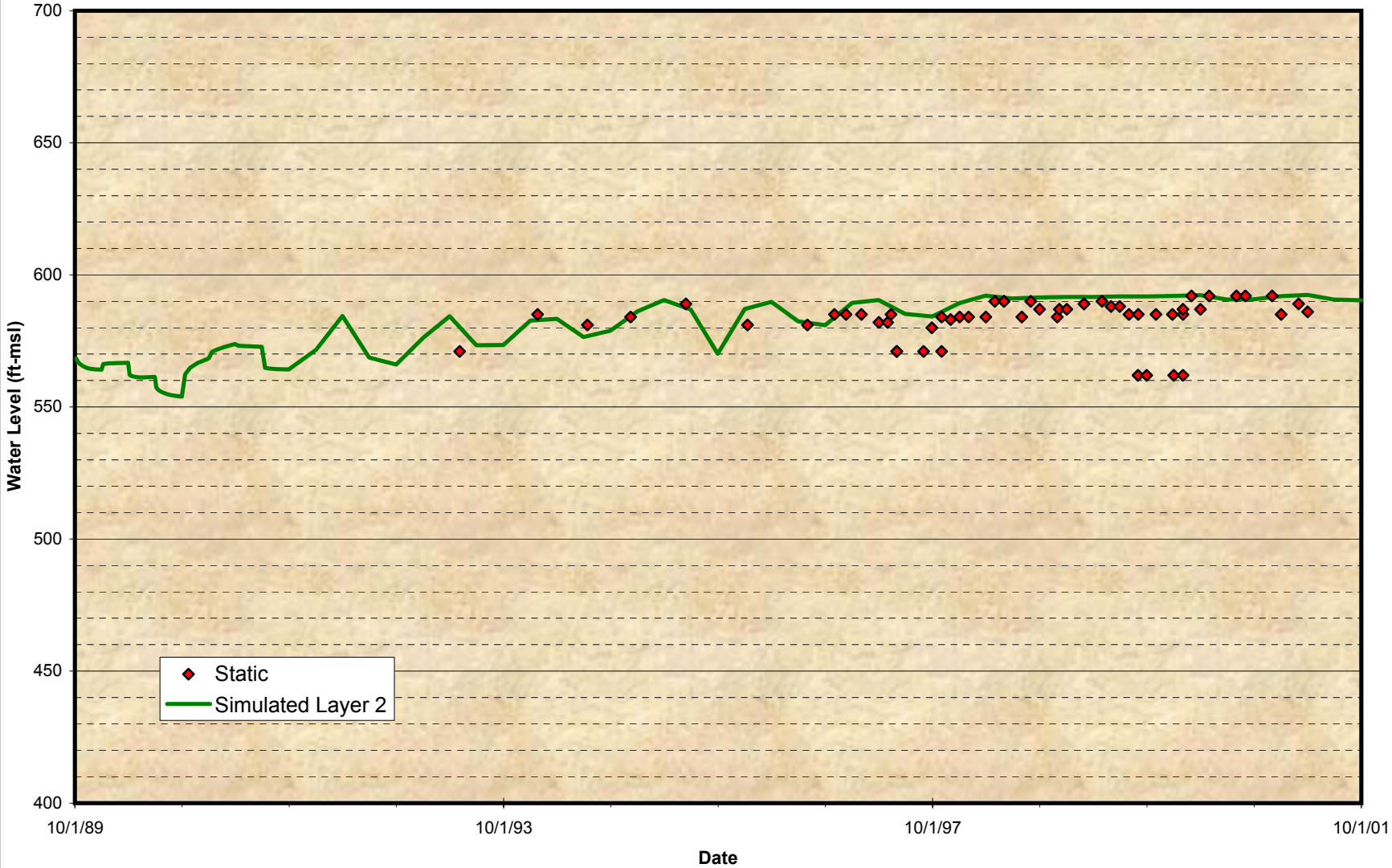
Figure 6-12 Comparison of Model Predicted Level and Observed Groundwater Level for Norco No. 11
