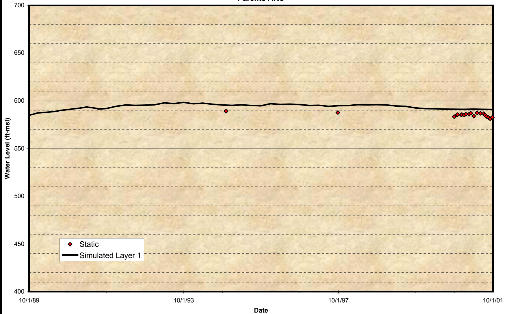
Figure 6-13 Comparison of Model Predicted Level and Observed Groundwater Level for a Private Well Parente ARC
