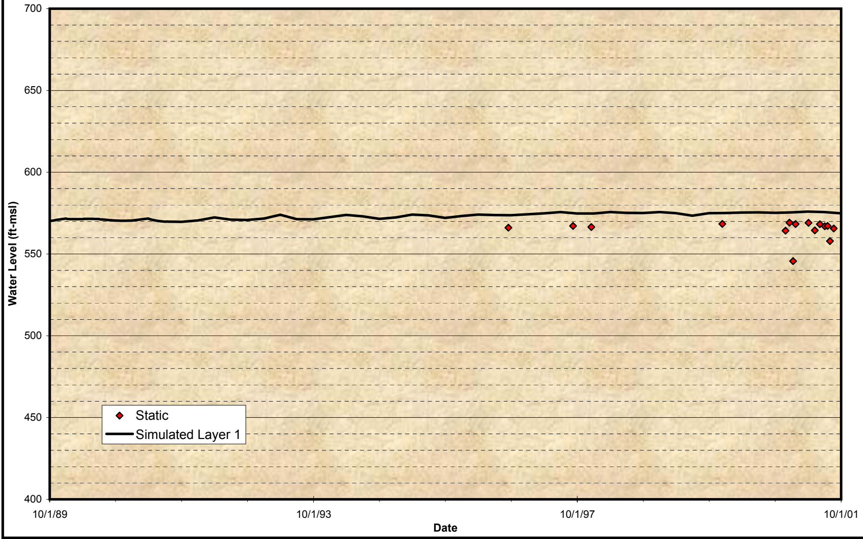
Figure 6-14 Comparison of Model Predicted Level and Observed Groundwater Level for a Private Well Excelsior
