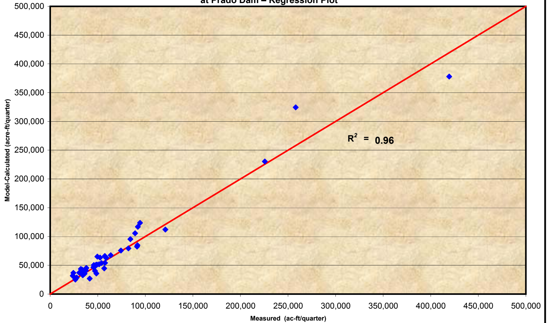
Figure 6-17b Comparison of Model-Projected and Observed Santa Ana River Discharge Time Histories at Prado Dam – Regression Plot
