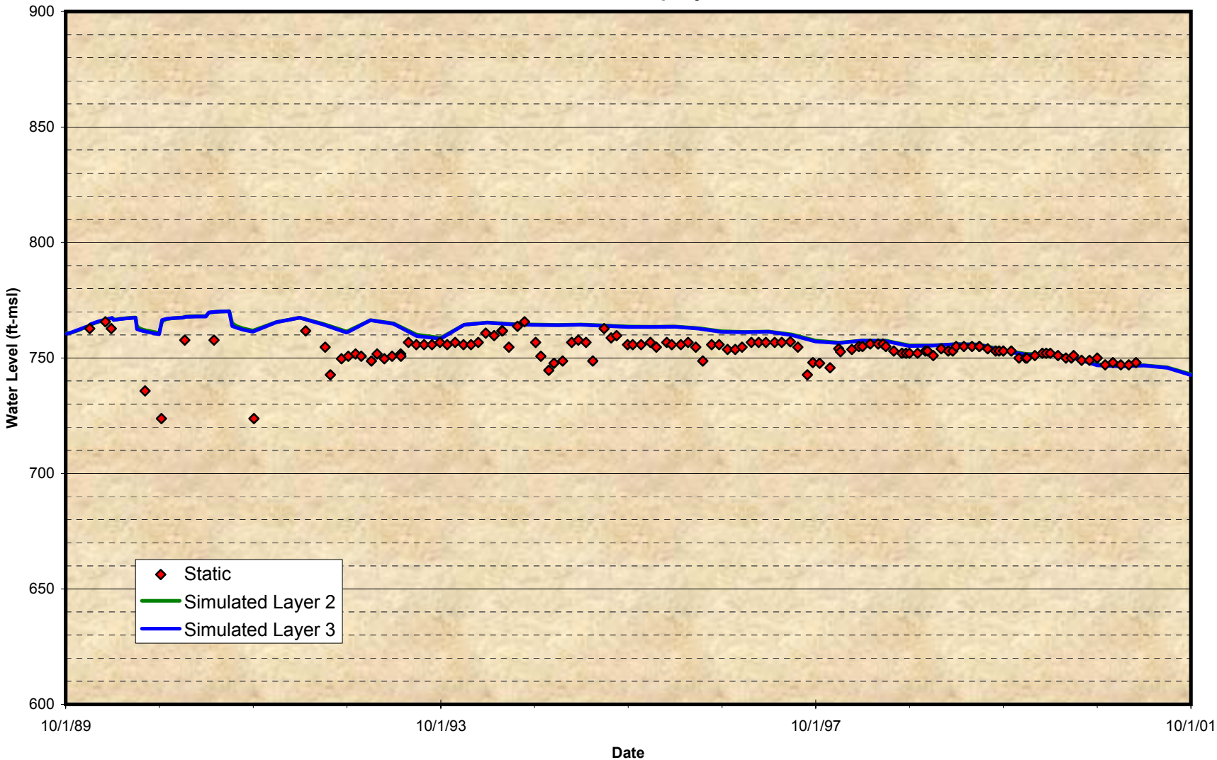
Figure 6-2 Comparison of Model Predicted Level and Observed Groundwater Level for Fontana Water Company No. F3A
