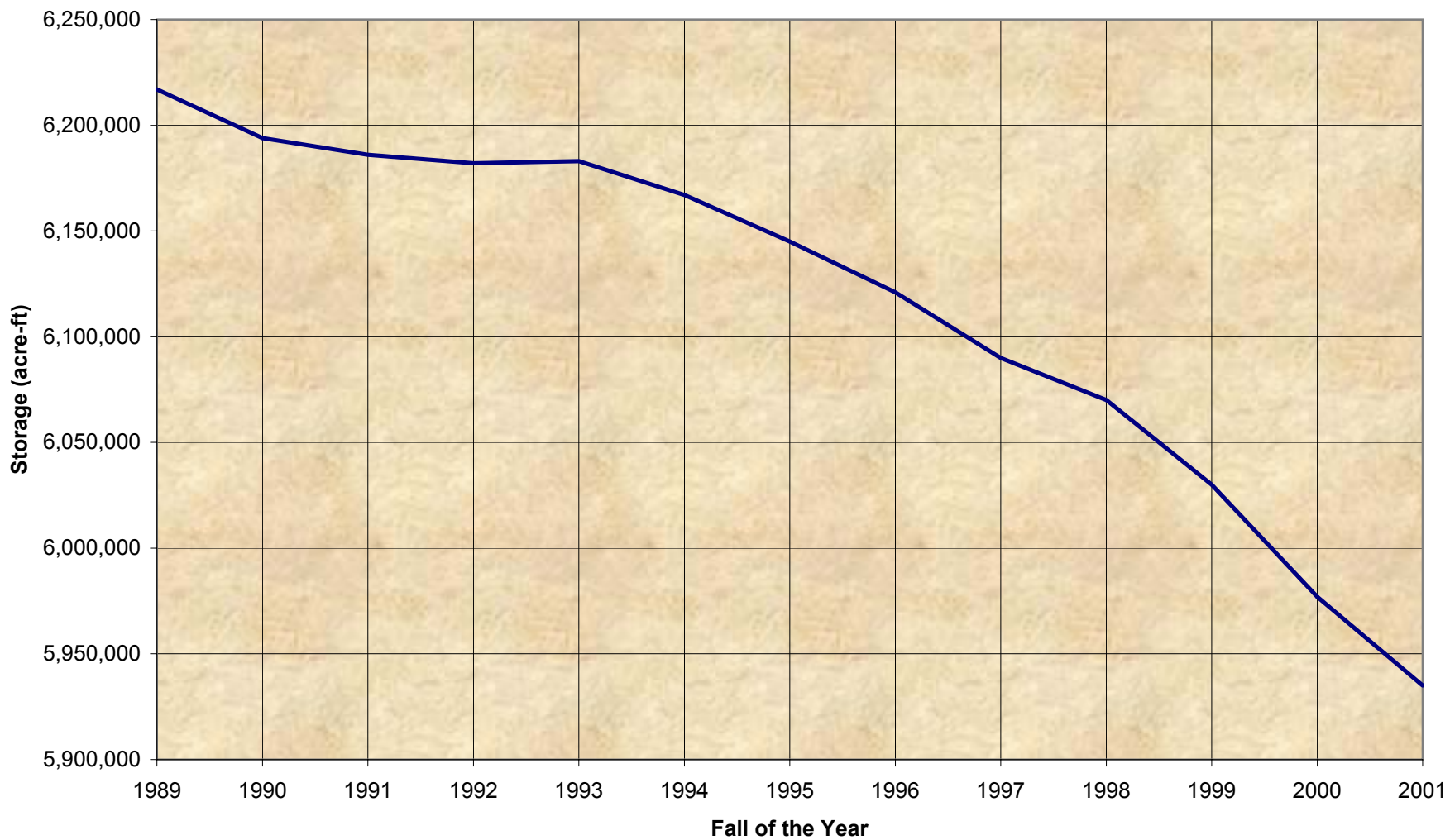
Figure 6-21 Time History of Total Storage in the Chino Basin Fall 1989 to Fall 2001
