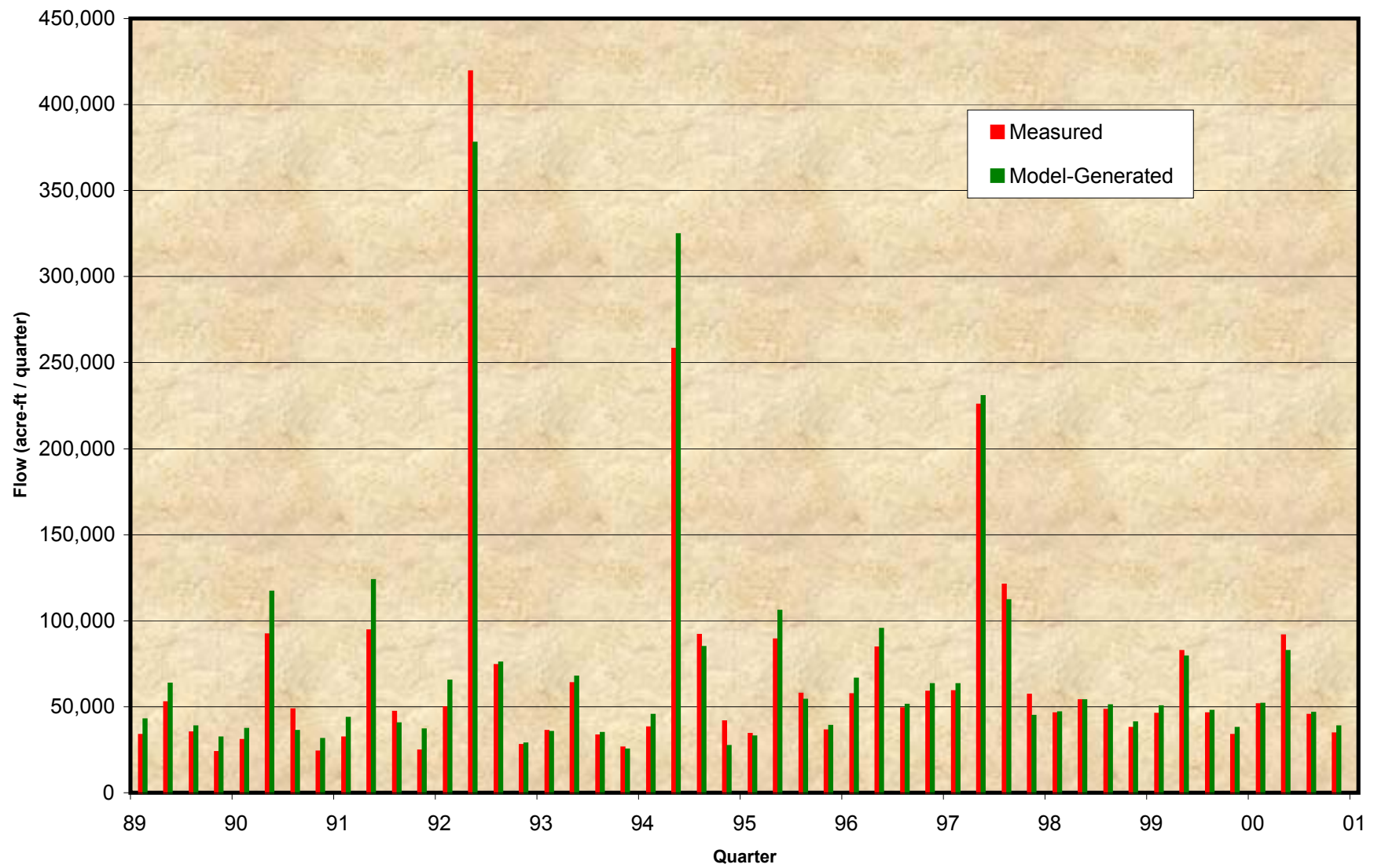
Figure 6-22 Comparison of Model-Projected and Observed Santa Ana River Discharge at Prado
