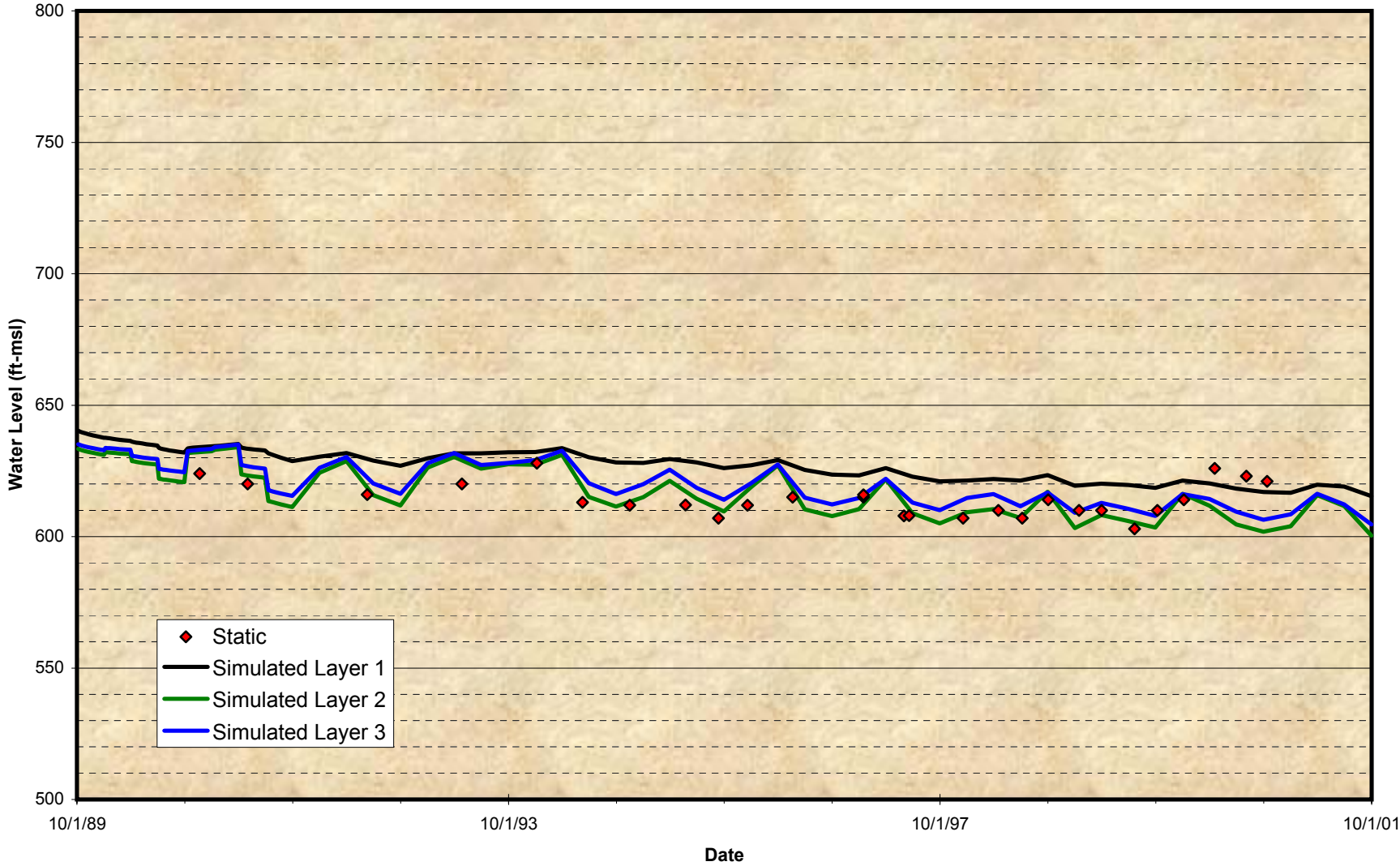
Figure 6-4 Comparison of Model Predicted Level and Observed Groundwater Level for Ontario No. 17
