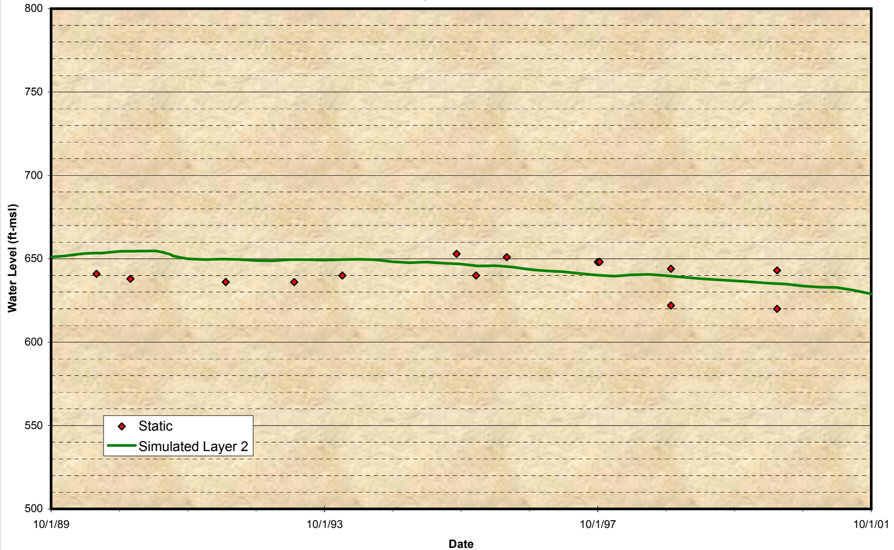
Figure 6-5 Comparison of Model Predicted Level and Observed Groundwater Level for Upland No. 3
