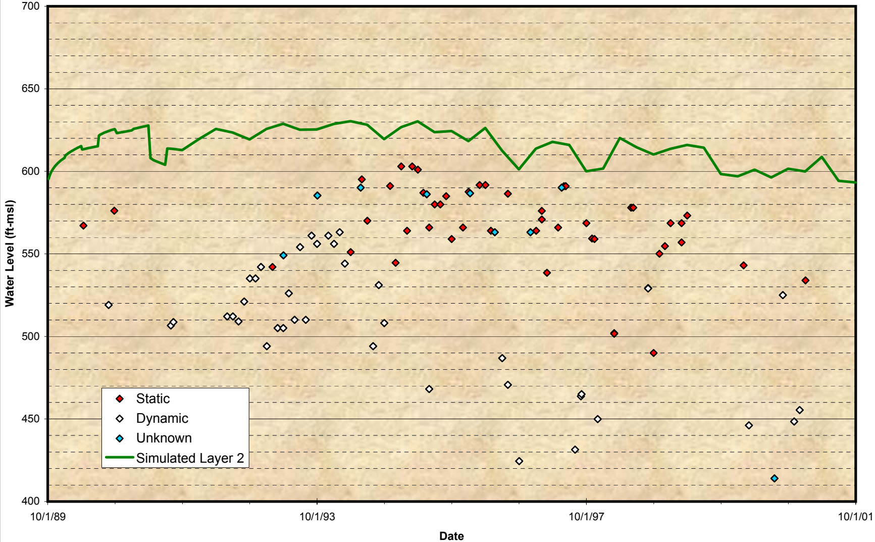
Figure 6-6 Comparison of Model Predicted Level and Observed Groundwater Level for Monte Vista No. 10
