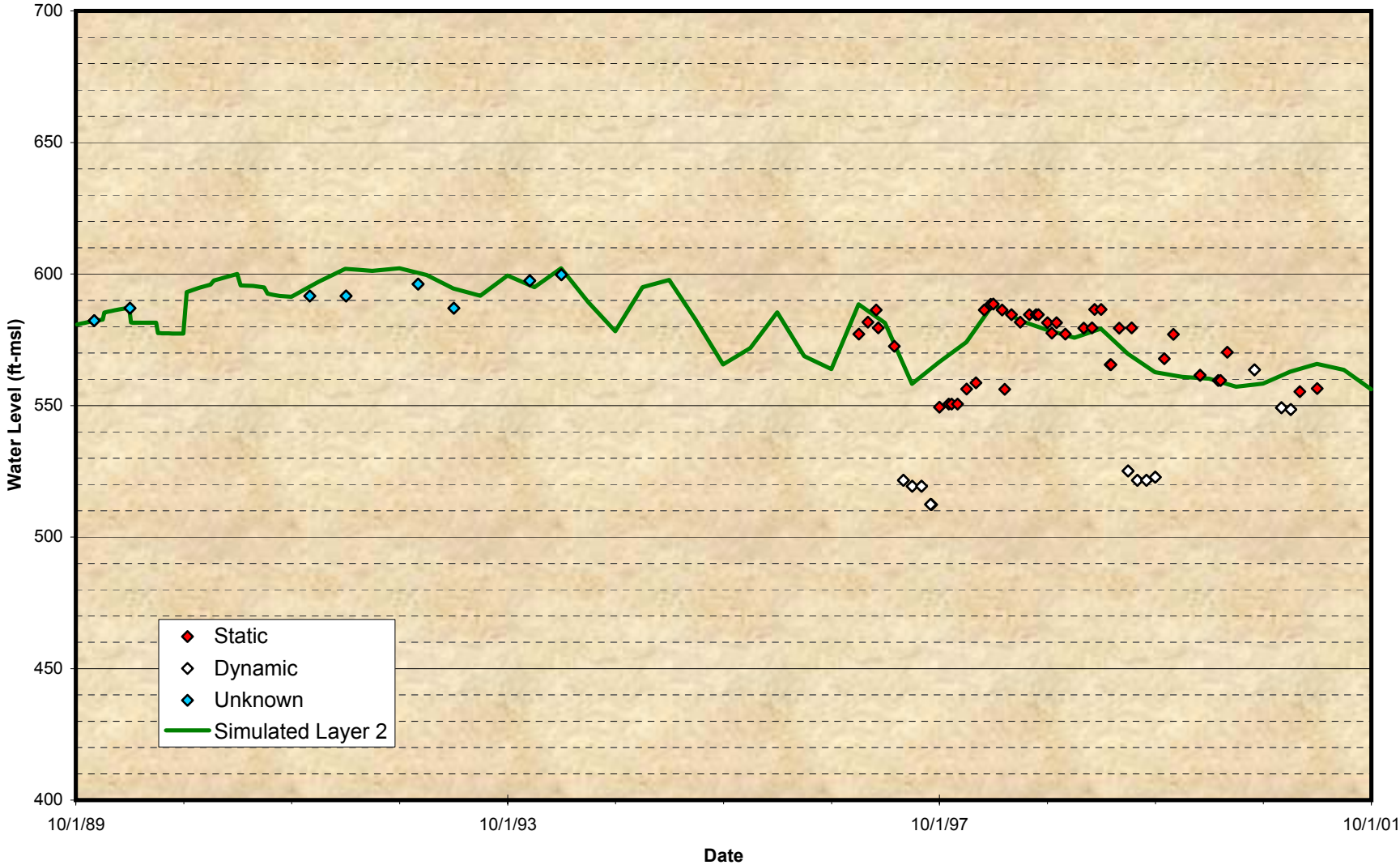
Figure 6-7 Comparison of Model Predicted Level and Observed Groundwater Level for Pomona No. 11
