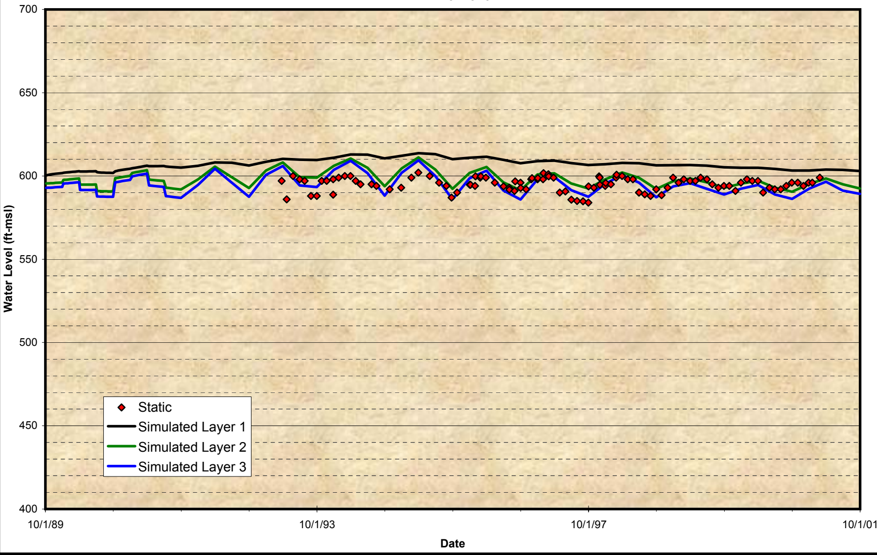
Figure 6-8 Comparison of Model Predicted Level and Observed Groundwater Level for Chino No. 9
