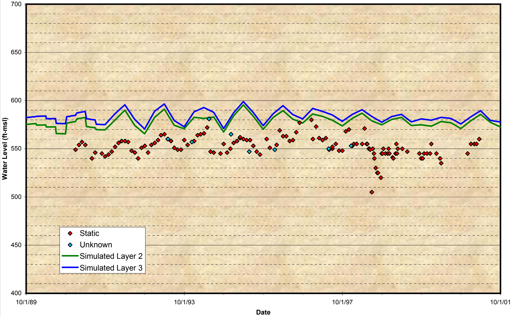
Figure 6-9 Comparison of Model Predicted Level and Observed Groundwater Level for Chino Hills No. 18A
