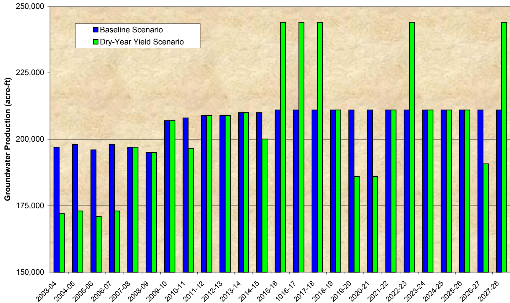
Figure 7-1 Chino Basin Groundwater Pumping Schedules for the Baseline and Dry-Year Yield Scenarios
