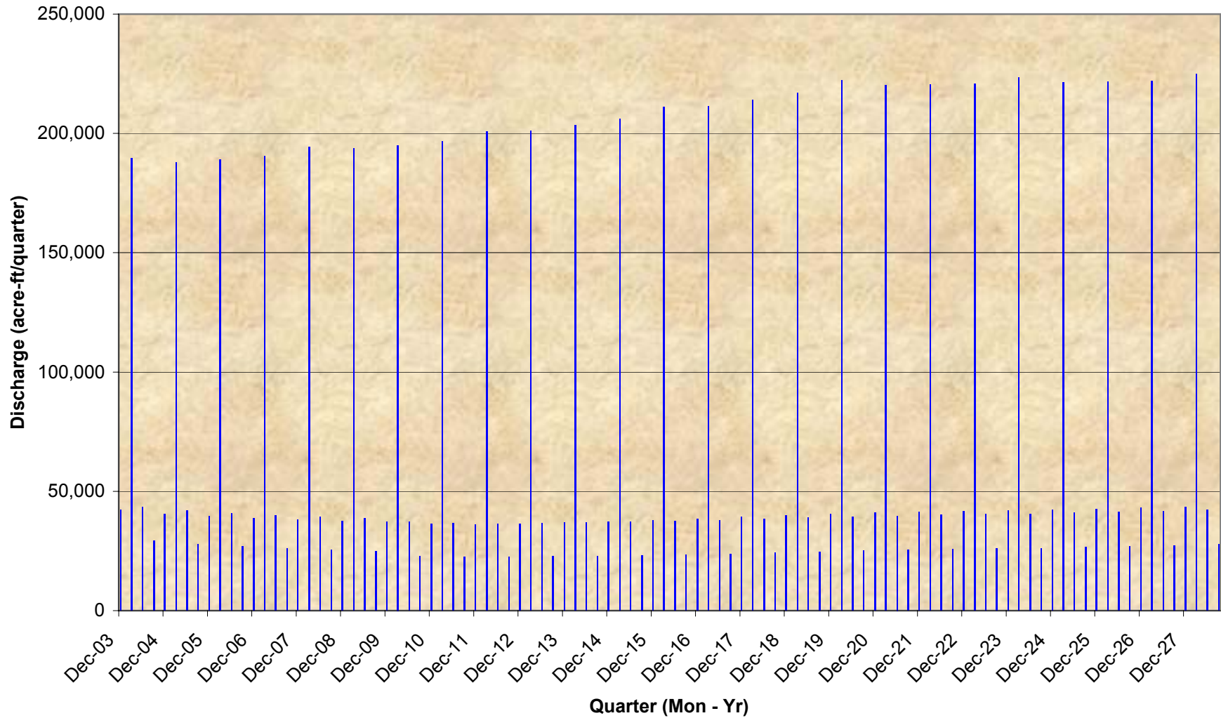
Figure 7-5 Projected Annual Time Histories of the Santa Ana River Discharge at Prado for the Baseline Scenario
