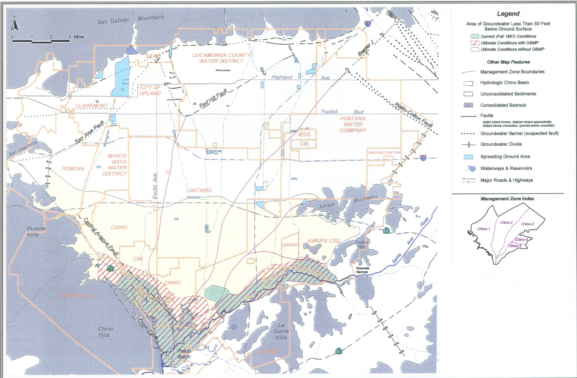
AREA IN SOUTHWEST CHINO BASIN (SAN BERNARDINO COUNTY) WITH HIGH LIQUEFACTION POTENTIAL
