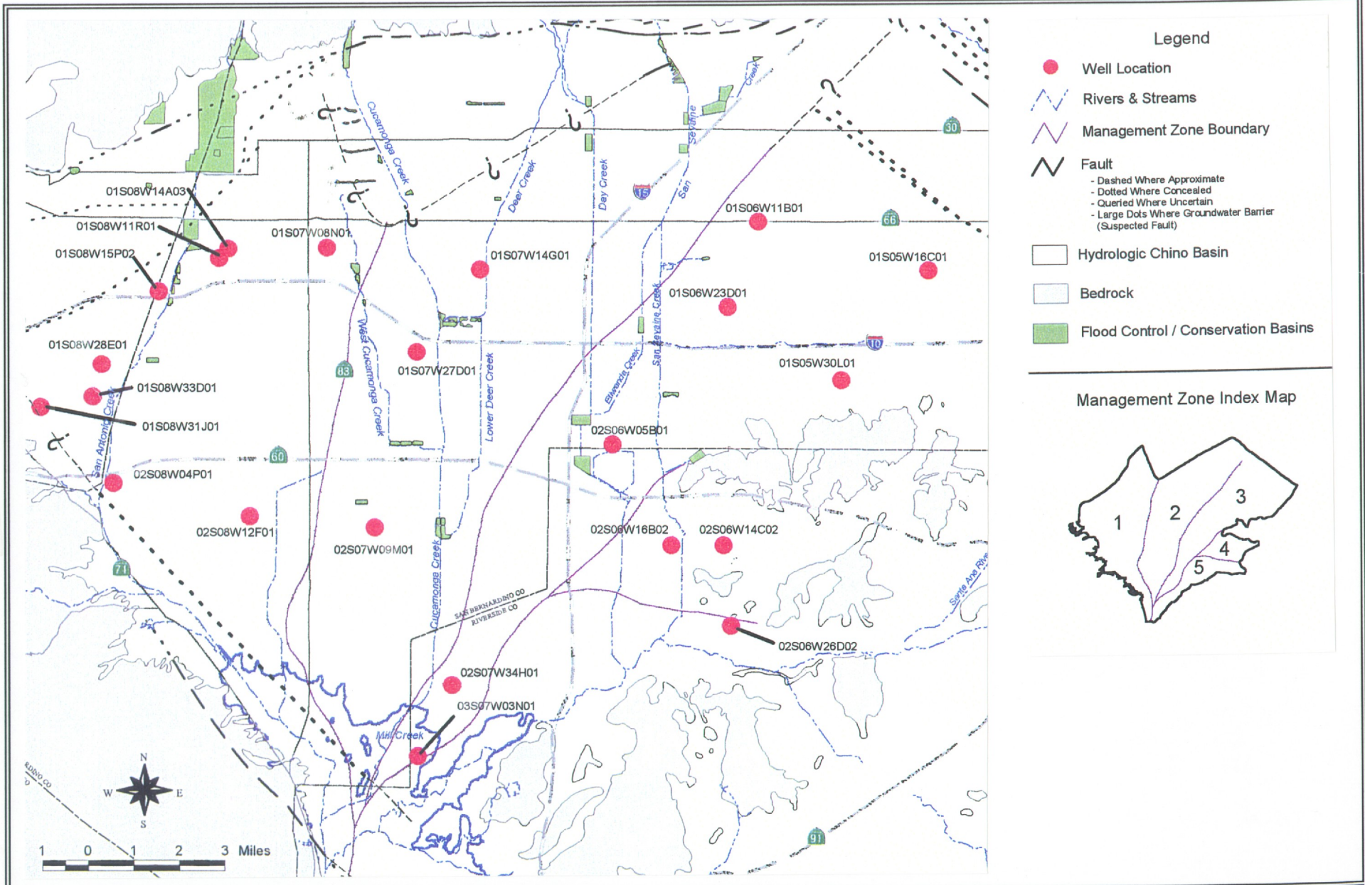
WELL LOCATION MAP FOR WATER LEVEL TIME HISTORIES
