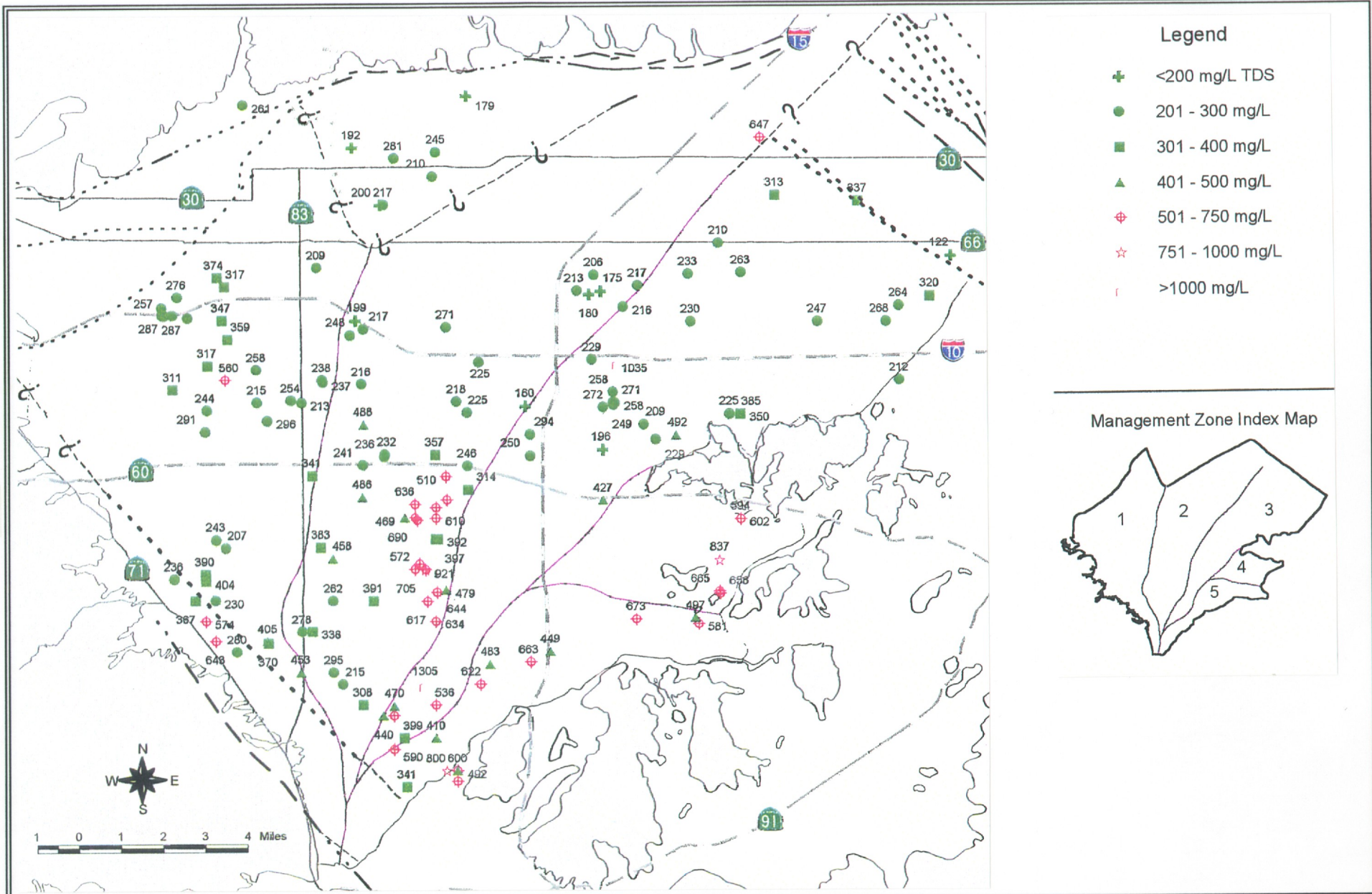
AVERAGE TDS CONCENTRATIONS (mg/L) IN THE CHINO BASIN - 1961 TO 1965
