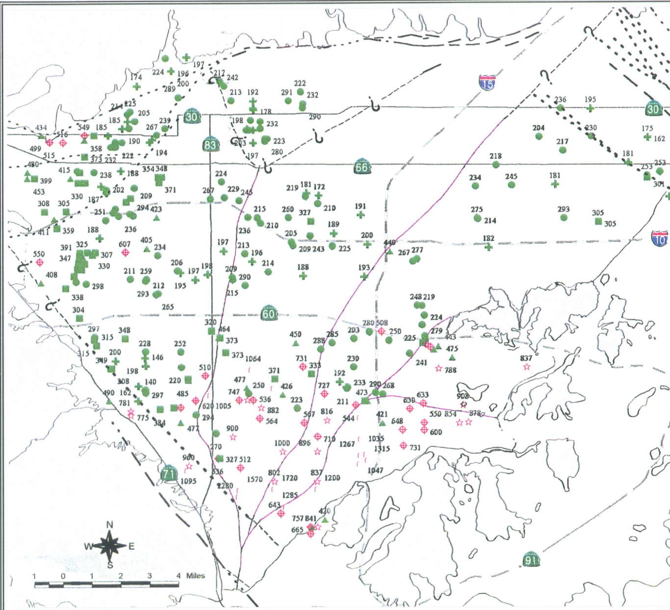
AVERAGE TDS CONCENTRATIONS (mg/L) IN THE CHINO BASIN - 1991 TO 1995
