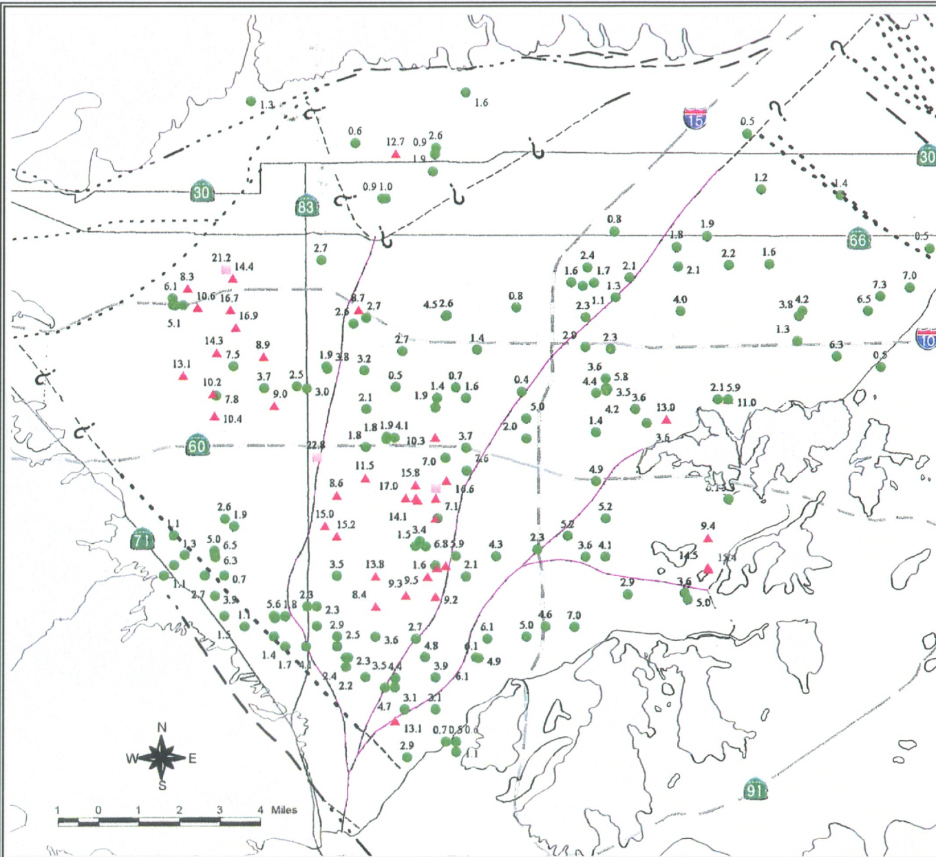
AVERAGE NITRATE-N CONCENTRATIONS (mg/L) IN THE CHINO BASIN - 1961 TO 1965
