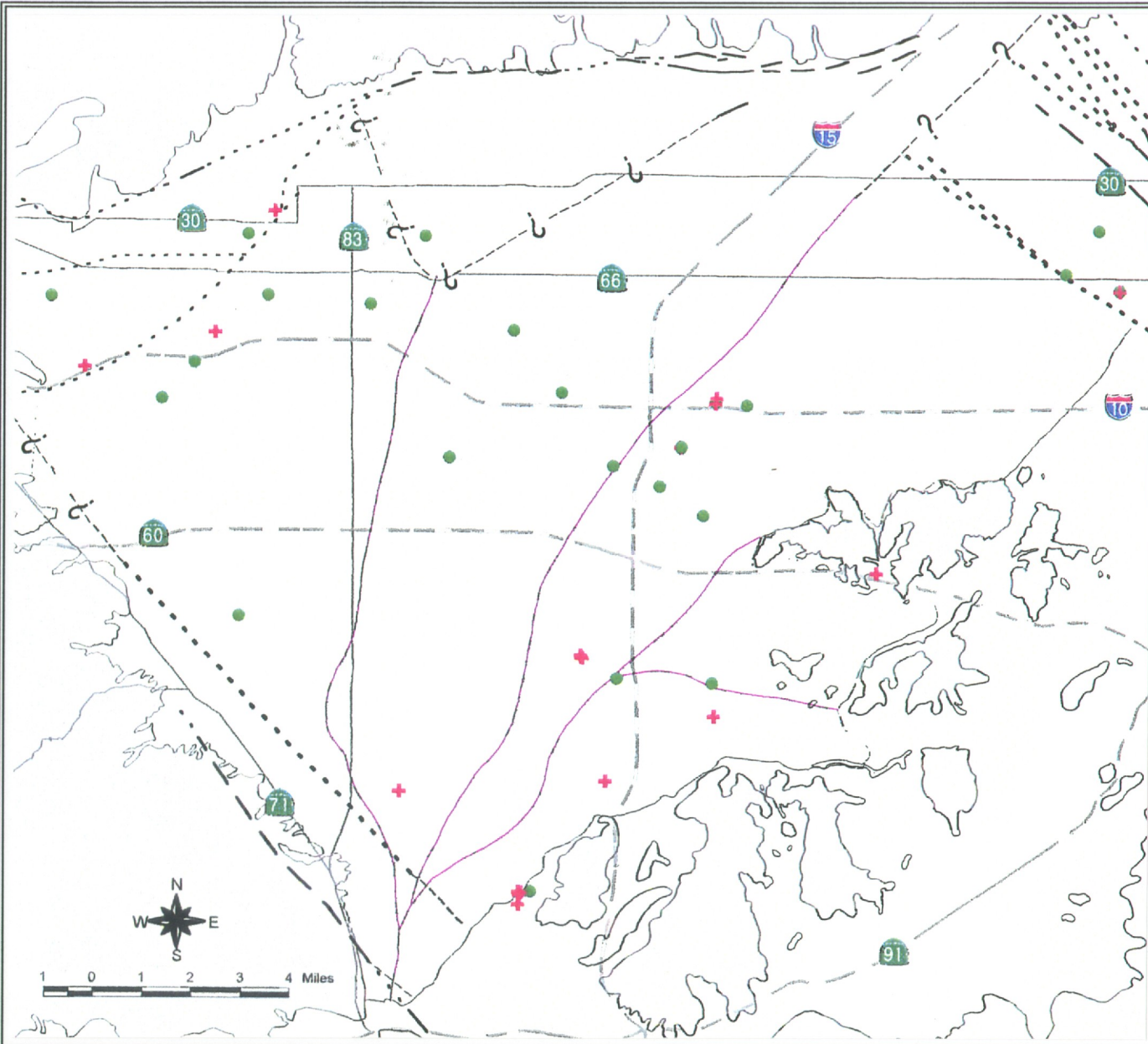
WELLS WITH ONE OR MORE HISTORICAL MANGANESE VALUES ABOVE 1/2 THE EXISTING MCL Source: OBMP Phase I Report, Figure 2-46
