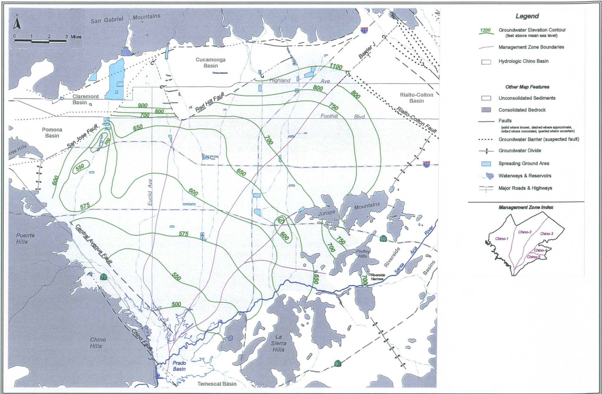
ESTIMATED GROUNDWATER ELEVATION FOR CURRENT (1997) CONDITIONS
