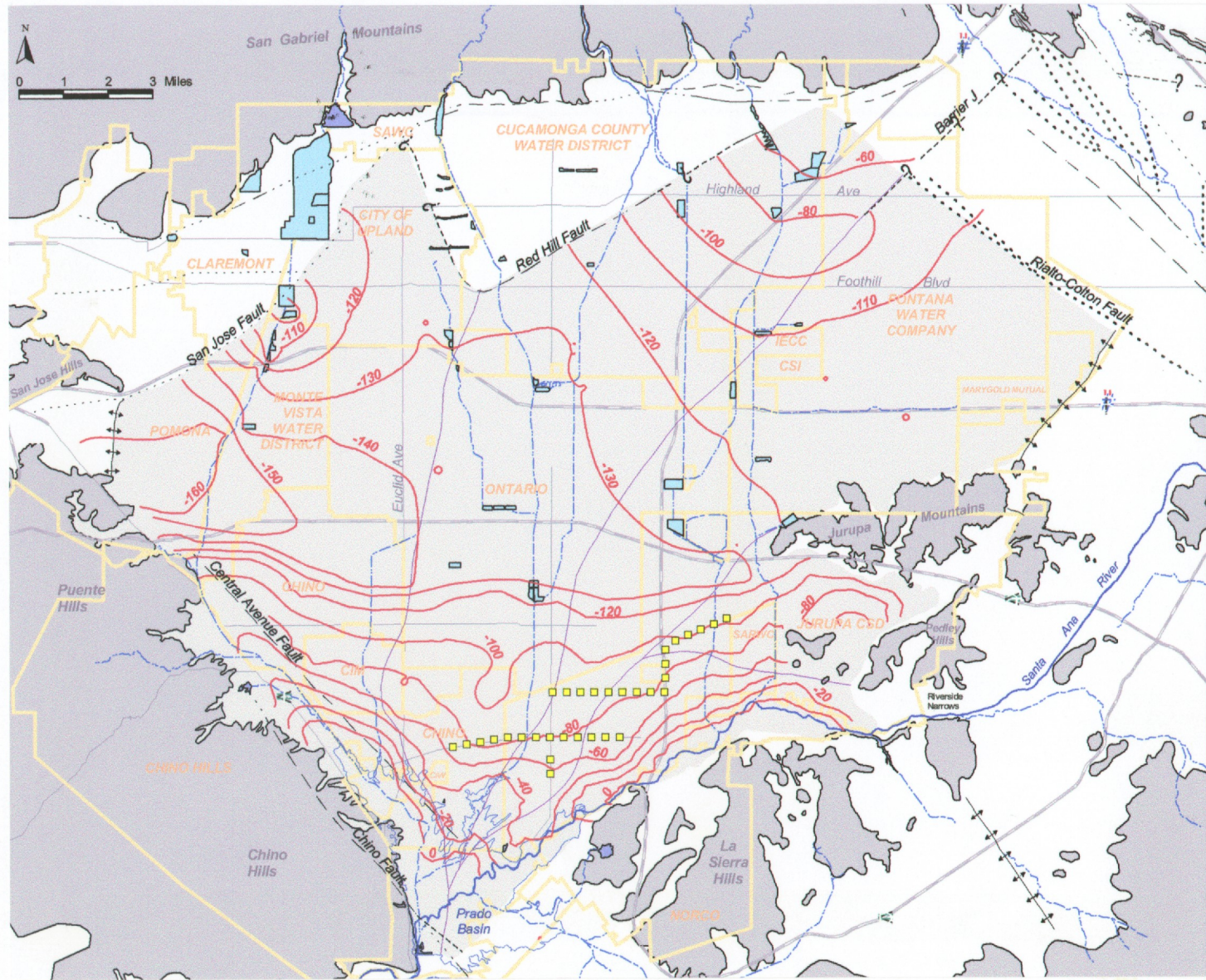
DIFFERENCE IN GROUNDWATER ELEVATIONS FROM NON-OBMP TO OBMP CONDITIONS FOR ULTIMATE CONDITIONS
