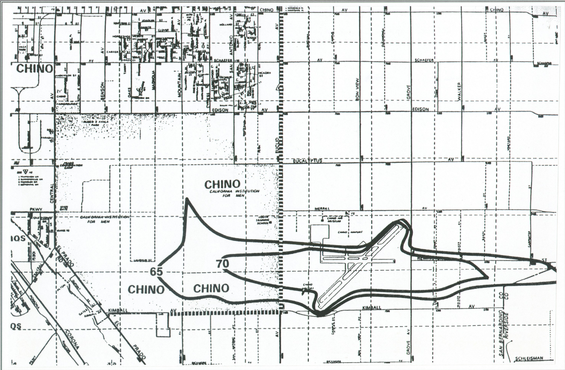
CHINO AIRPORT FUTURE CNEL NOISE CONTOURS
