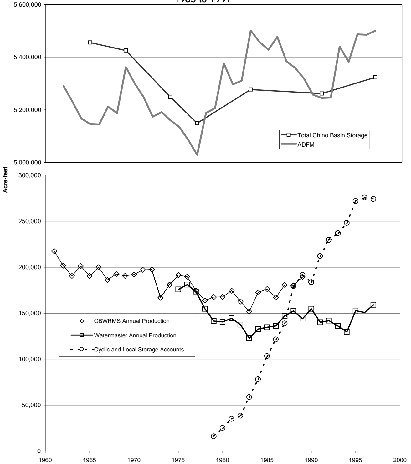
Figure 2-28 Estimated Groundwater Storage Compared to Average Production and Storage Accounts in the Chino Basin 1965 to 1997
