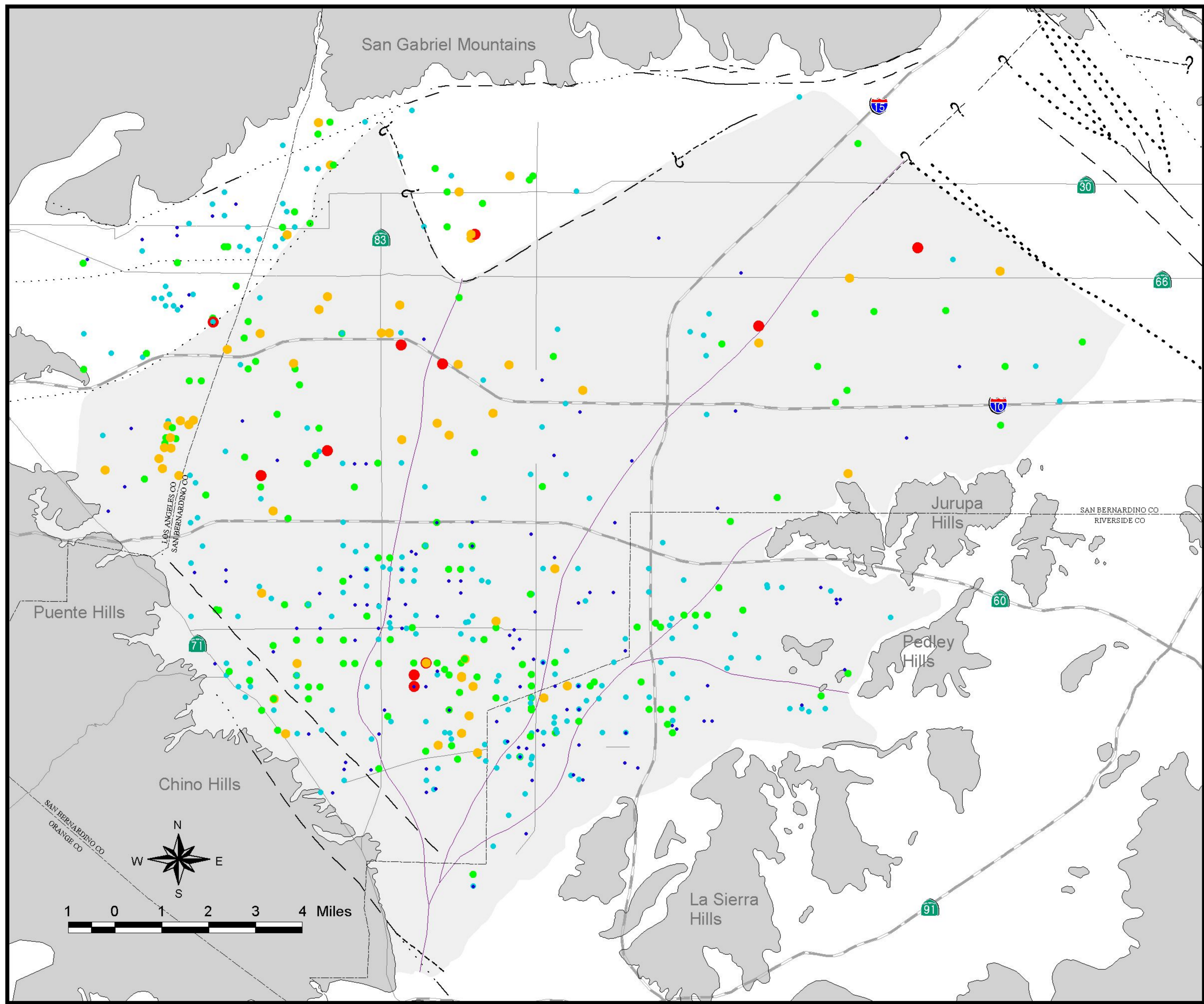
Figure 2-33 1971 Annual Production Estimates by Well from CBWRMS
