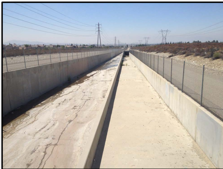
Field photo showing the location of the proposed improvement to the existing channel to increase storm water capture
